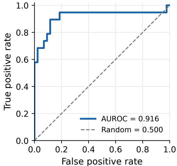
ROC curve
