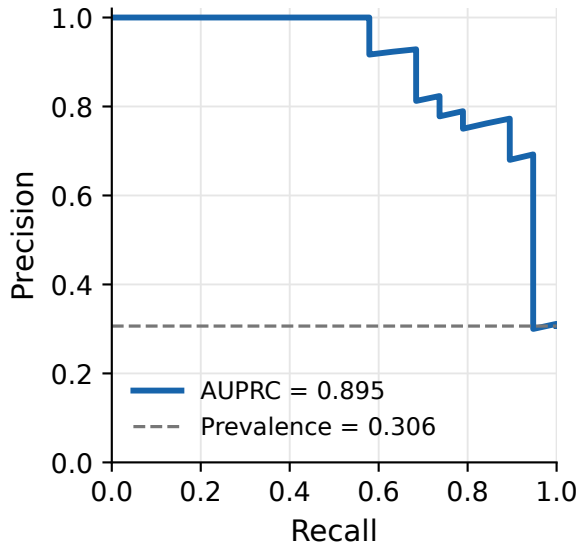
Precision-recall curve
