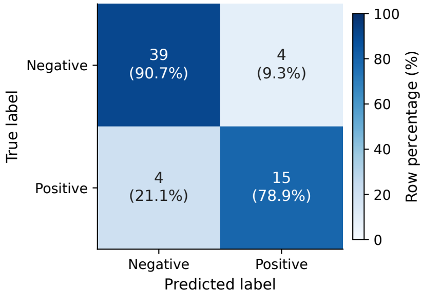
Confusion matrix
