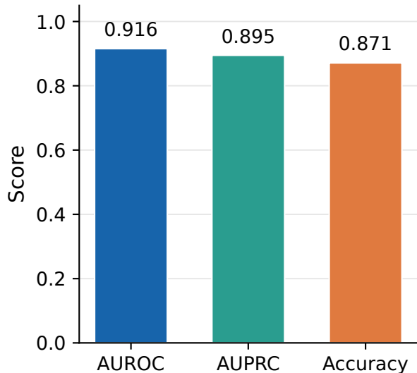
Classification performance
