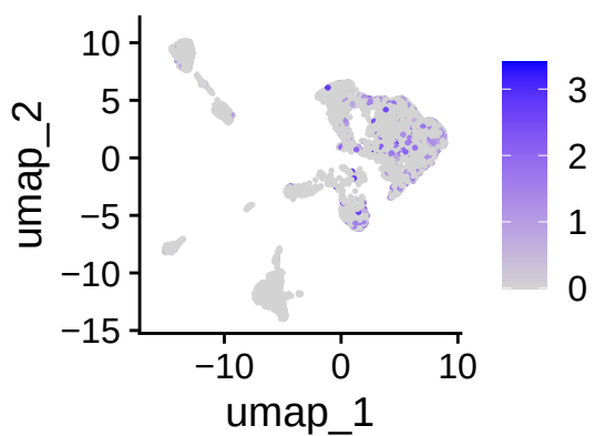
TMEM183A
