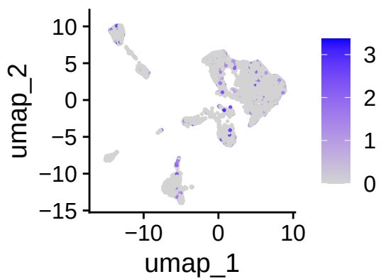
PRR11
