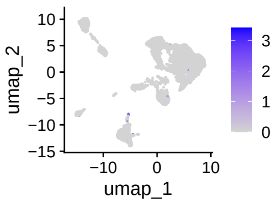
SHC2
