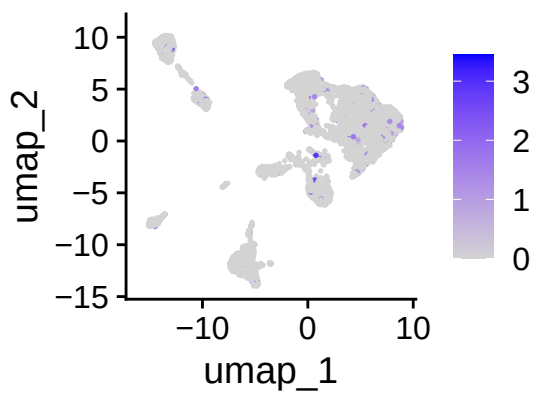
TMEM183A
