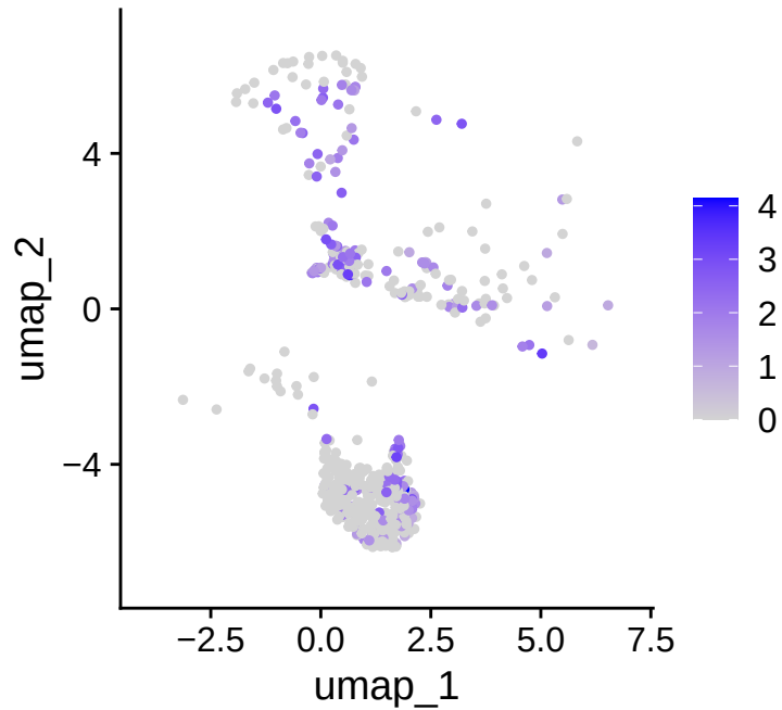
CDKN1A
