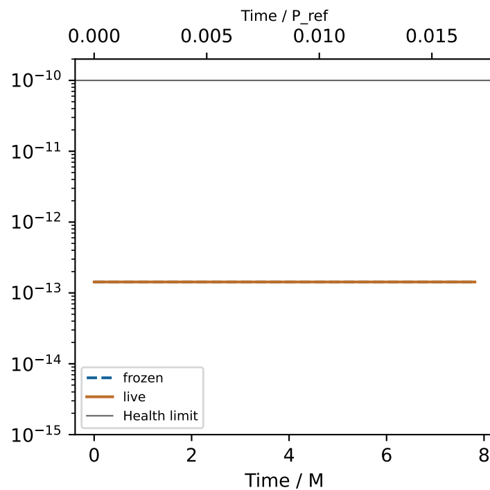
Relative rest-mass error
