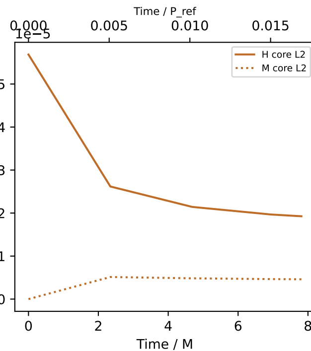
Live constraints ( r \leq 100M )
