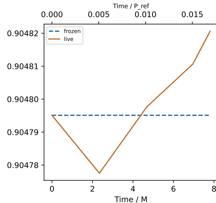
Frozen orbit error
