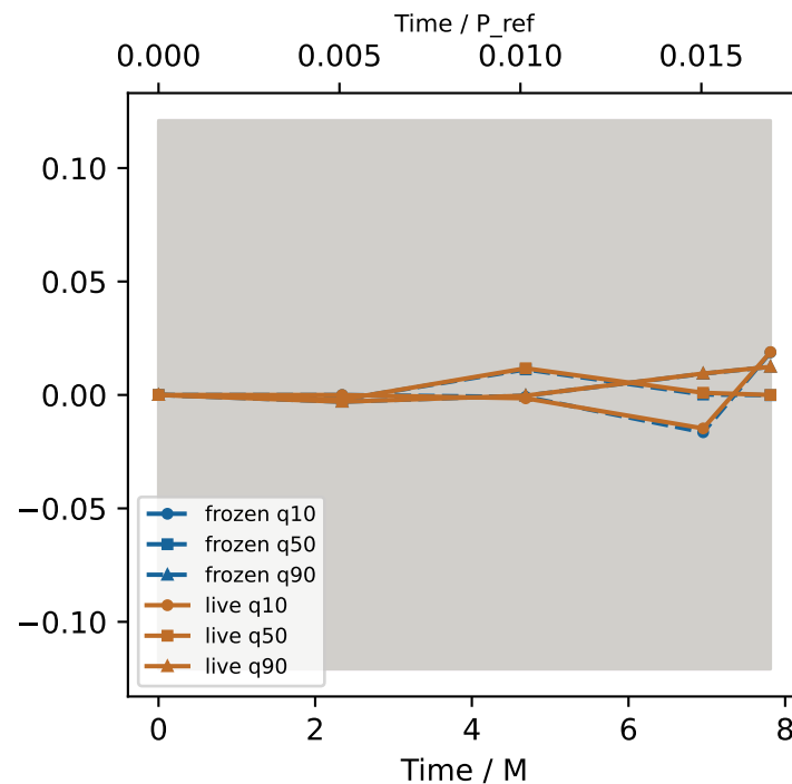
Live constraints ( r \leq 100M )
