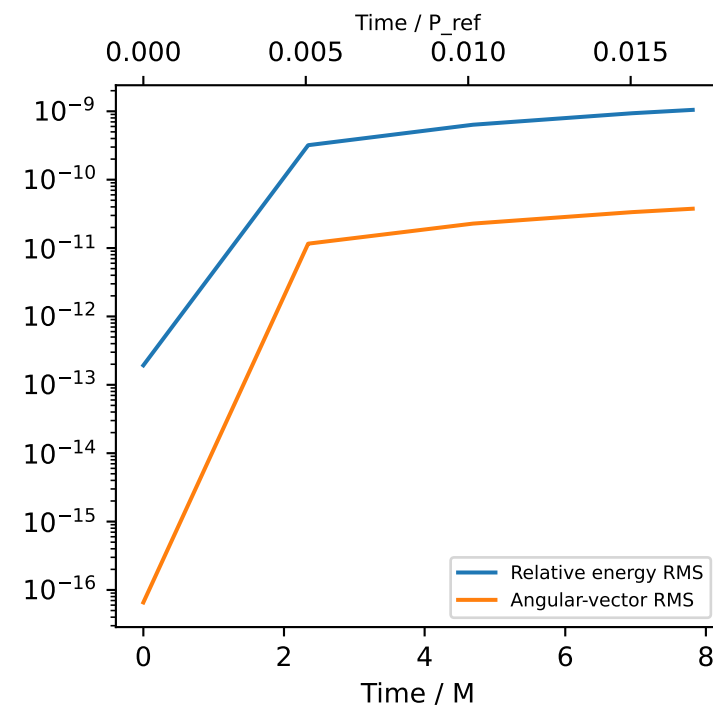
Frozen orbit error
