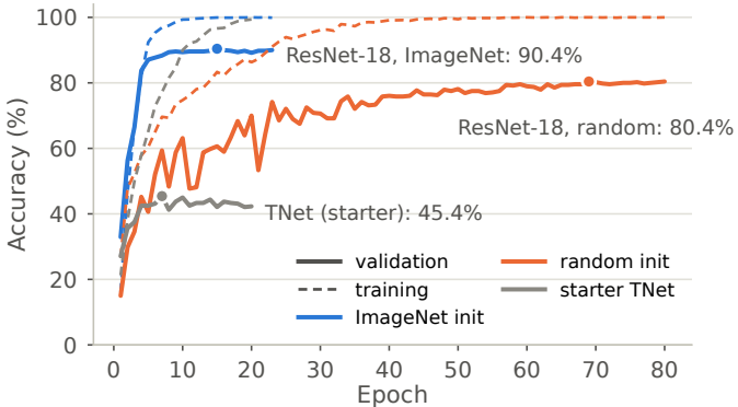
(a) Initialization, ResNet-18 vs. starter TNet
