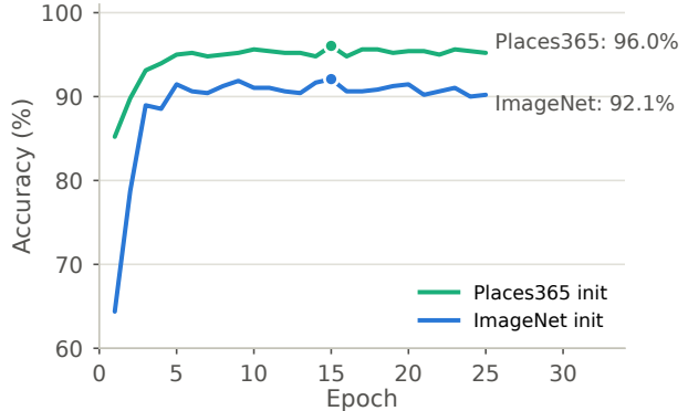
(b) Pretraining source, ResNet-50, same recipe
