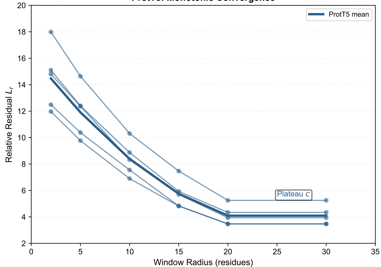
ProtT5: Monotonic Convergence
