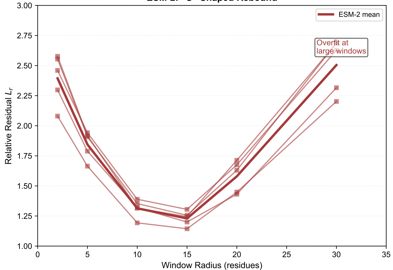
ESM-2: "U" Shaped Rebound
