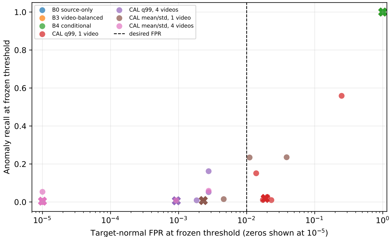
Operating-point reliability: seed-balanced scorer/direction cells
