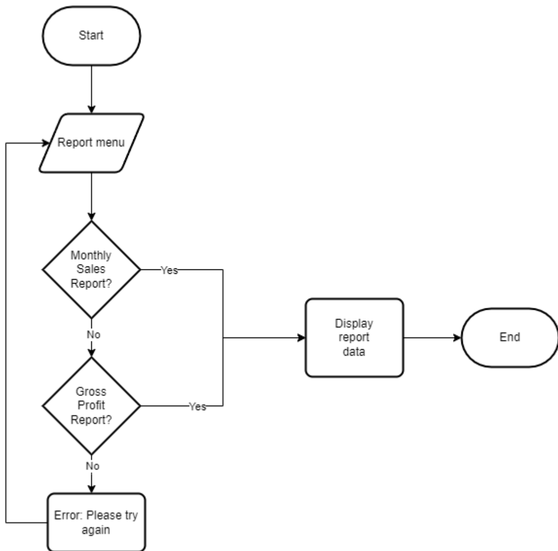
Figure 3.6: Report
