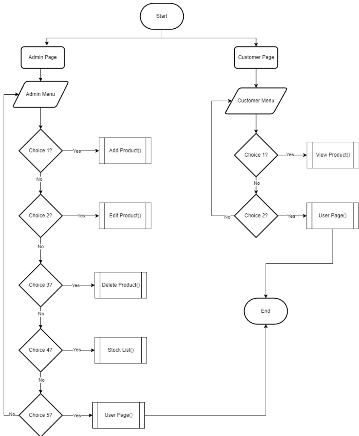
Figure 3.2: Product Management
