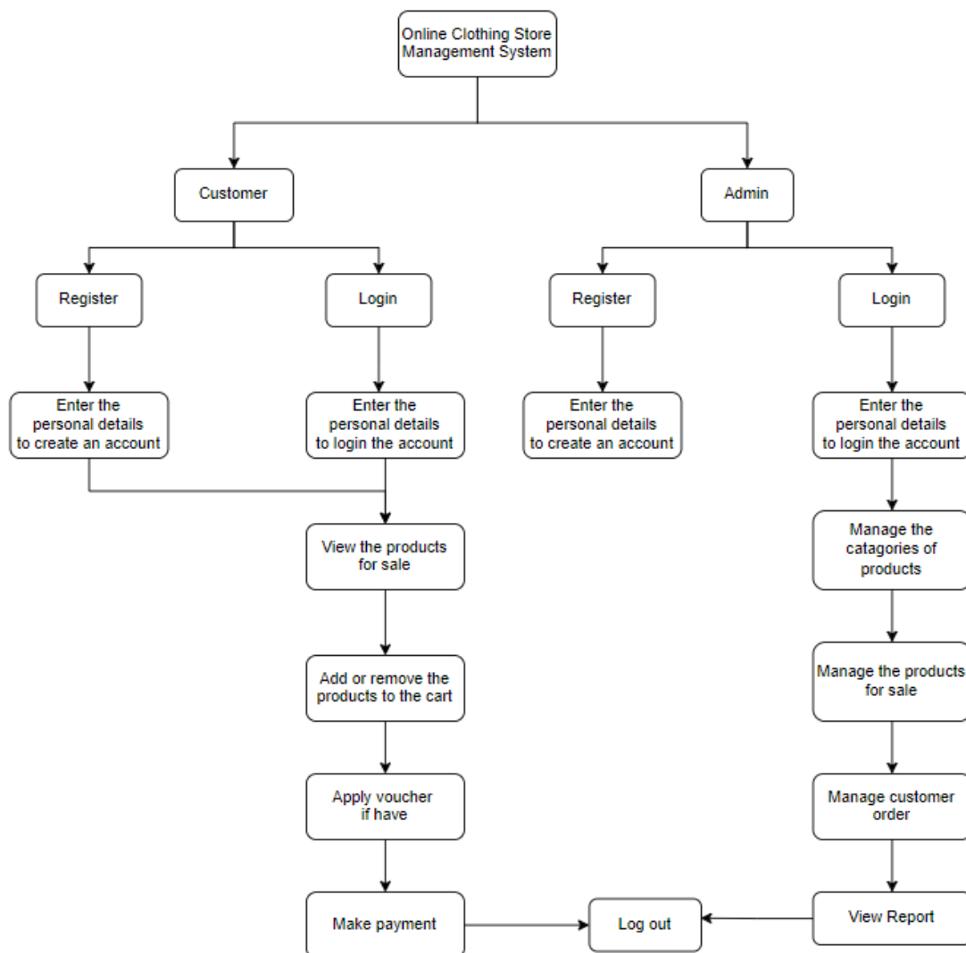
Figure 2.1: Structure Chart
