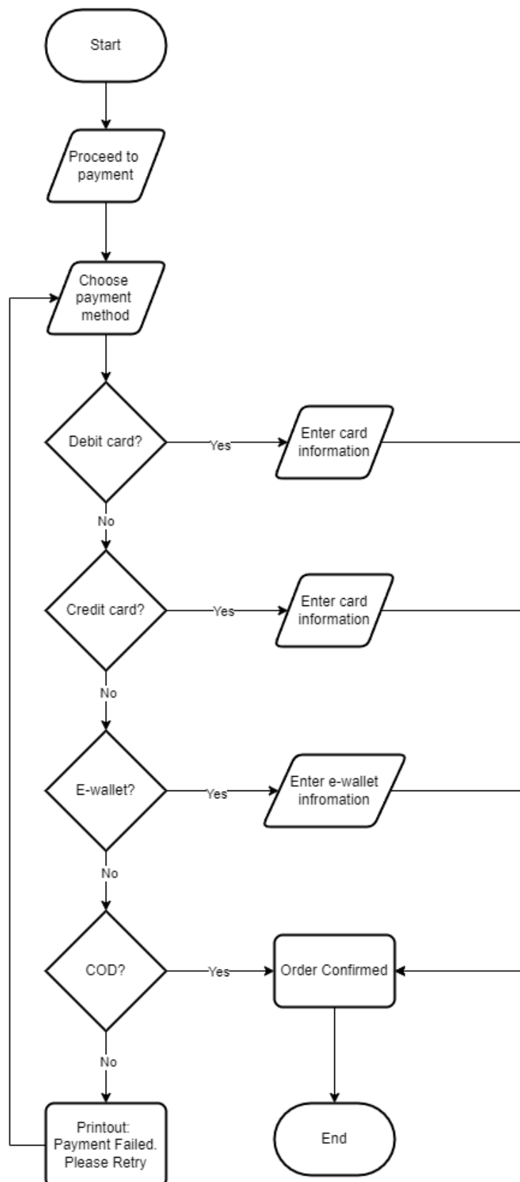
Figure 3.5: Payment
