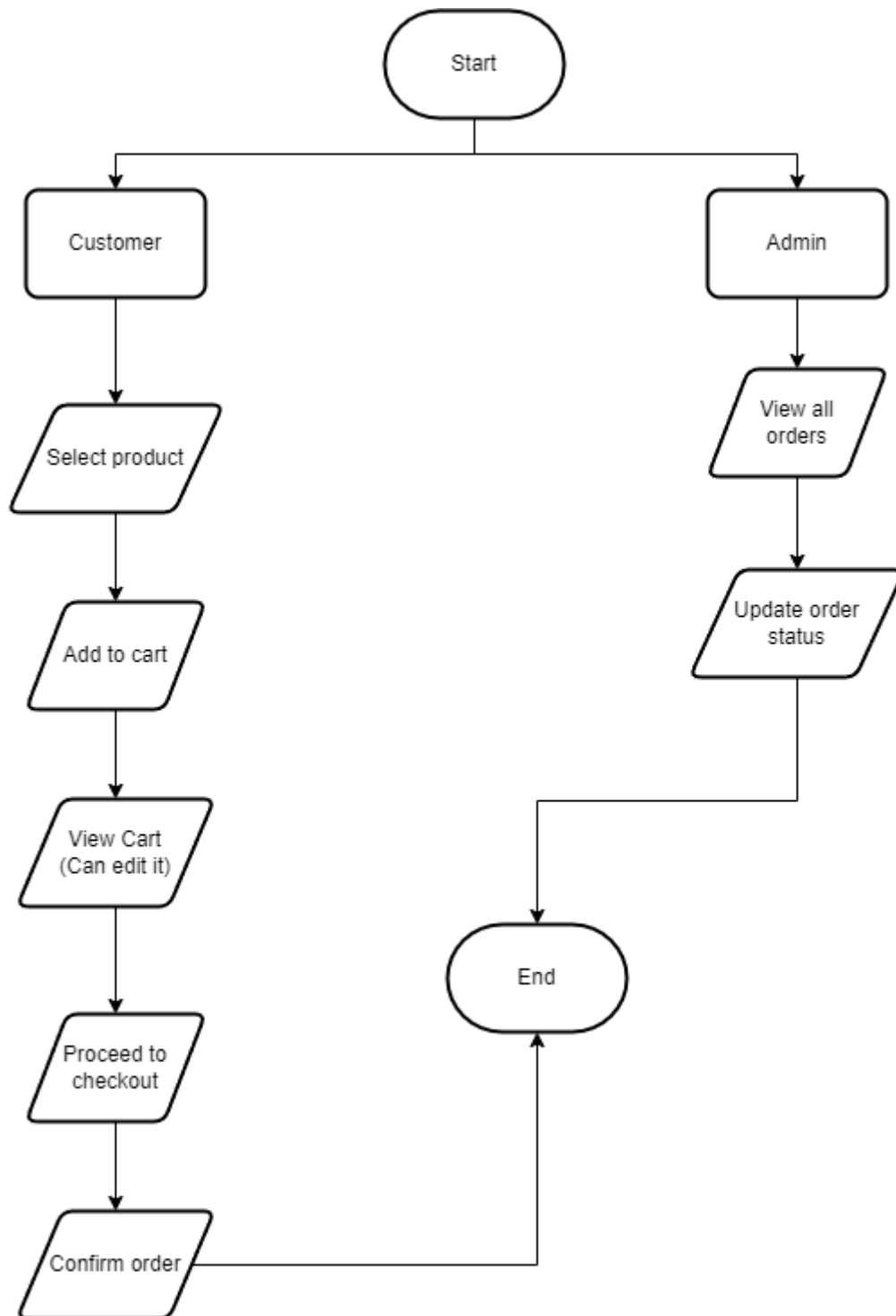
Figure 3.3: Order Management
