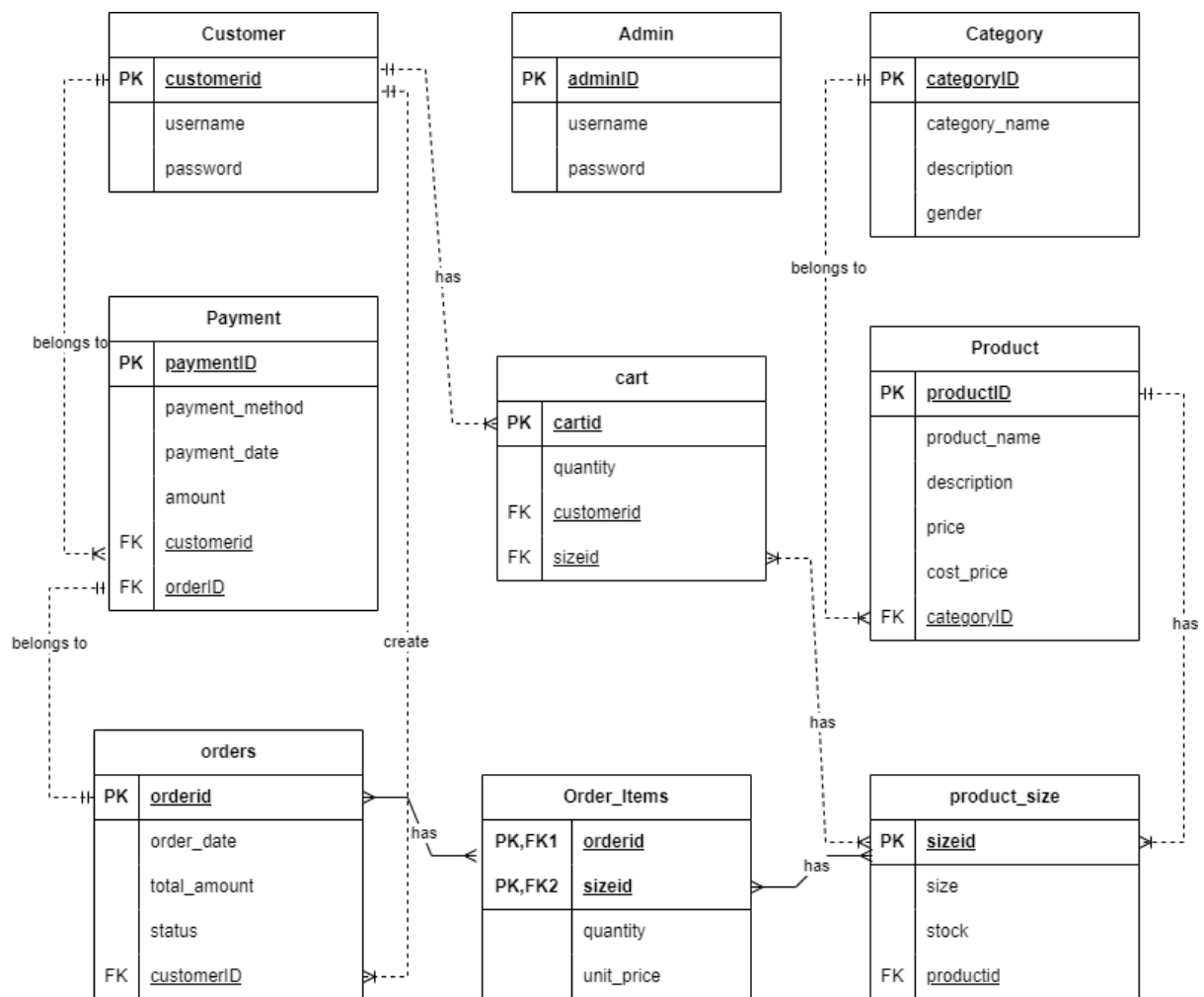
Figure 3.7: ERD
