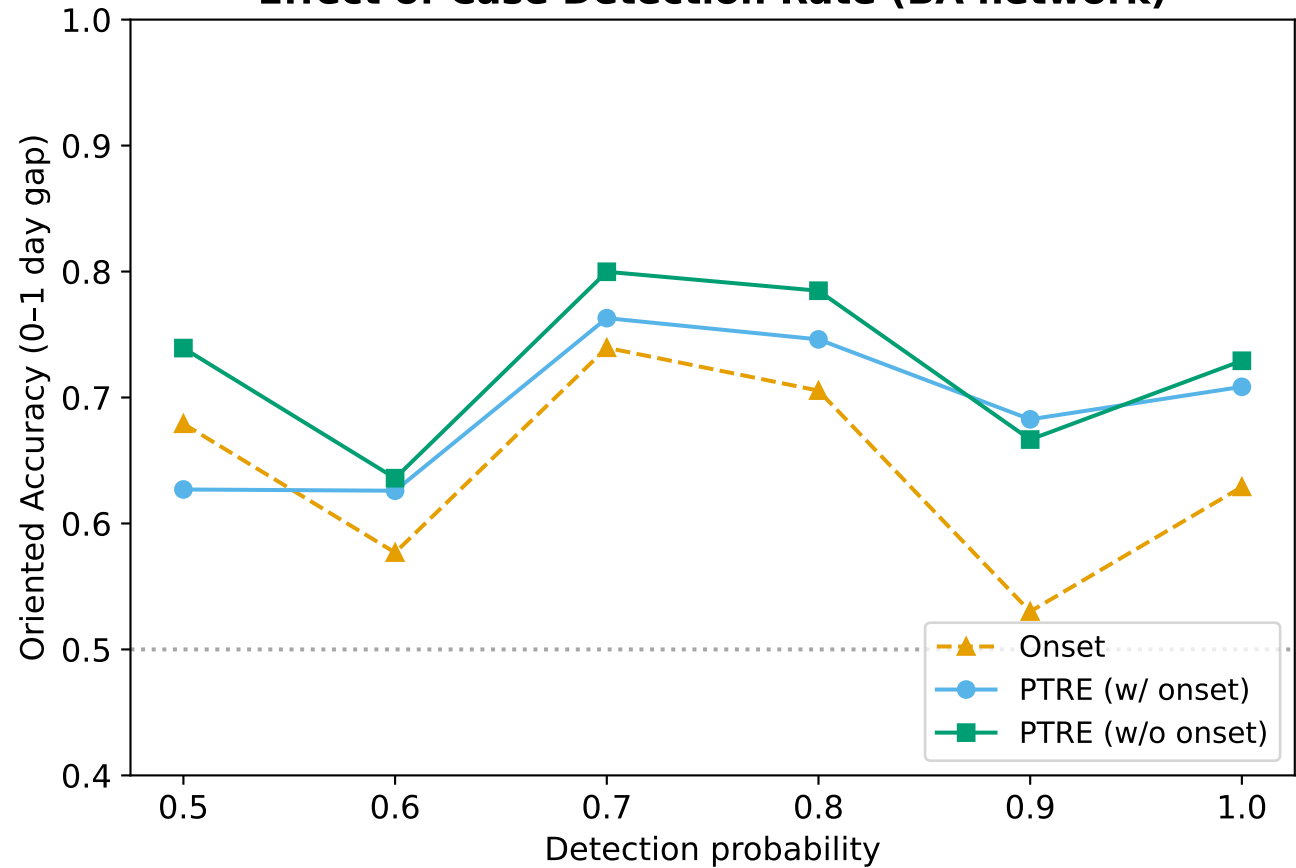
Effect of Case Detection Rate (BA network)
