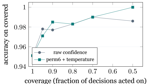
(b) Risk-coverage: abstain on the least confident.
