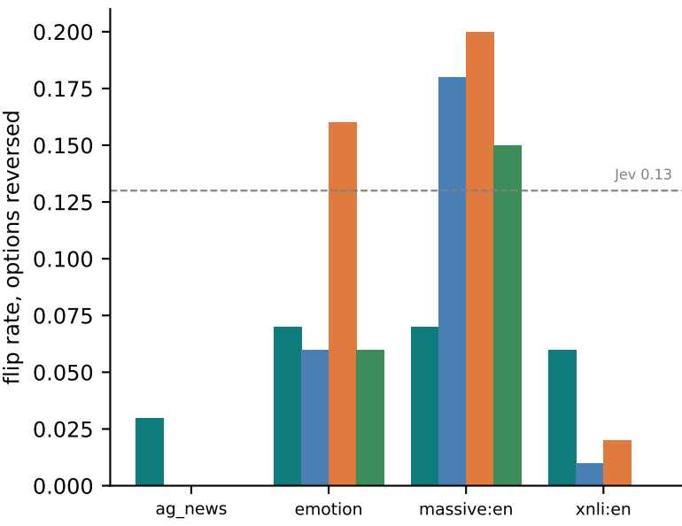
F · Option-order robustness (first 100 rows)
