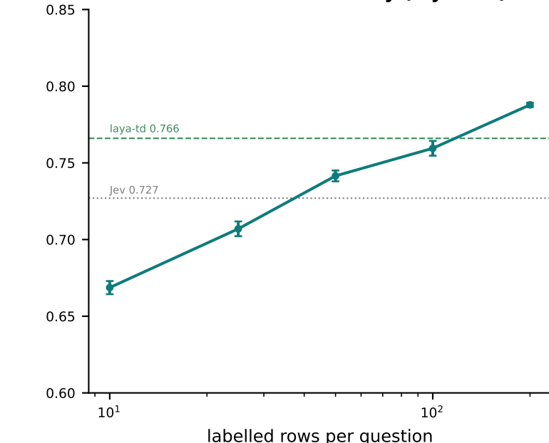
U · Probe data efficiency (layer 26)
