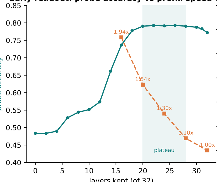
V · Early readout: probe accuracy vs prefill speed-up (4B)
