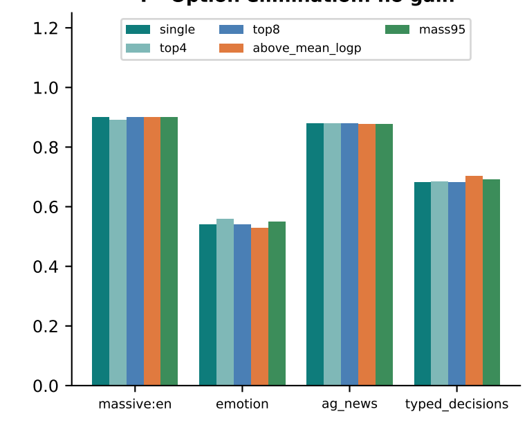
Y · Option elimination: no gain
