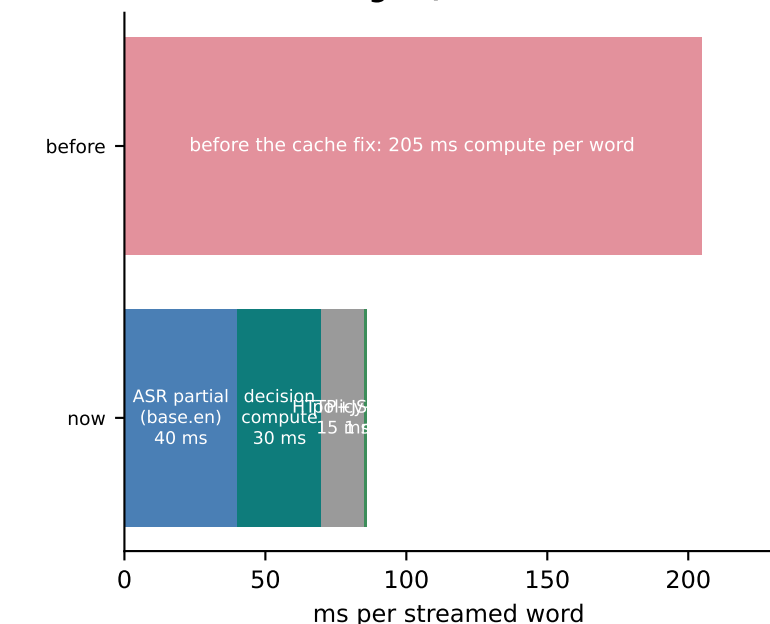
N · Per-word budget (~85 ms word → action)
