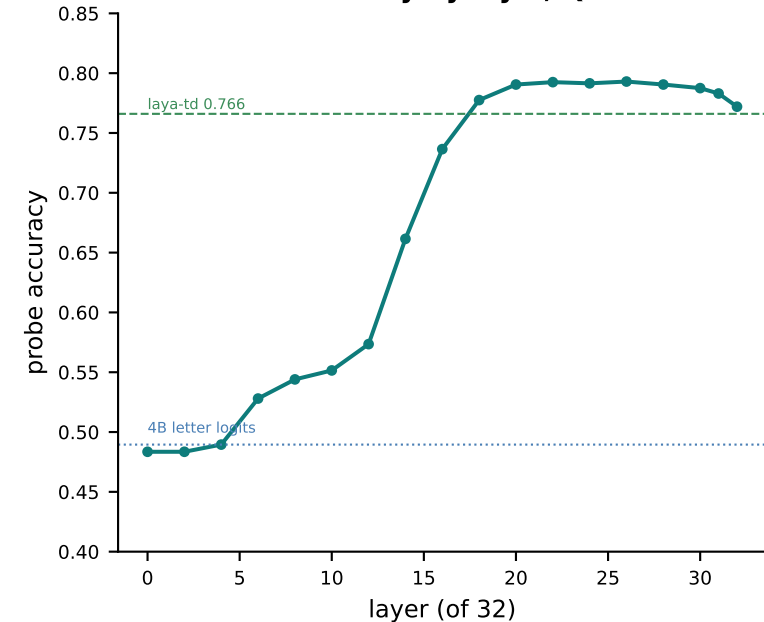
T · Probe accuracy by layer, Qwen3.5-4B
