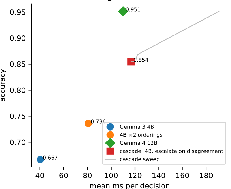
O · Small → large cascade: not worth it
