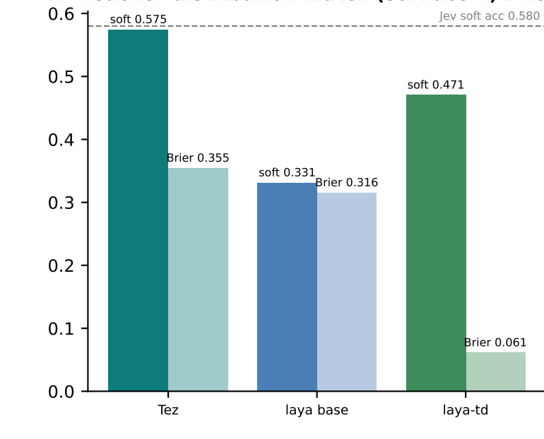
R · Teacher-distribution match (soft acc ↑, Brier ↓)
