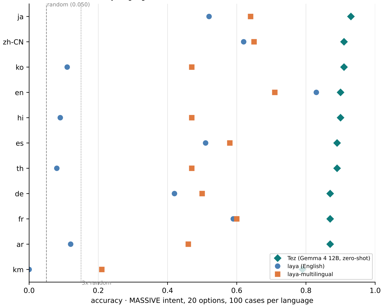
Every language, one frozen decoder vs two trained encoders
