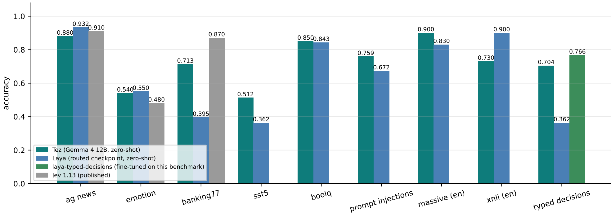
Same rows, same machine: Tez vs Laya (Jev bars are third-party published, not measured here)
