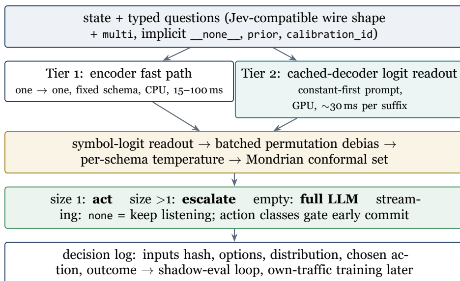
Figure 13: Two tiers, one contract. v1 is a harness around a frozen model; the evidence says post-hoc calibration is enough and that the frozen 12B (or a 4B with batched permutations) already reproduces and exceeds the published open baseline.
