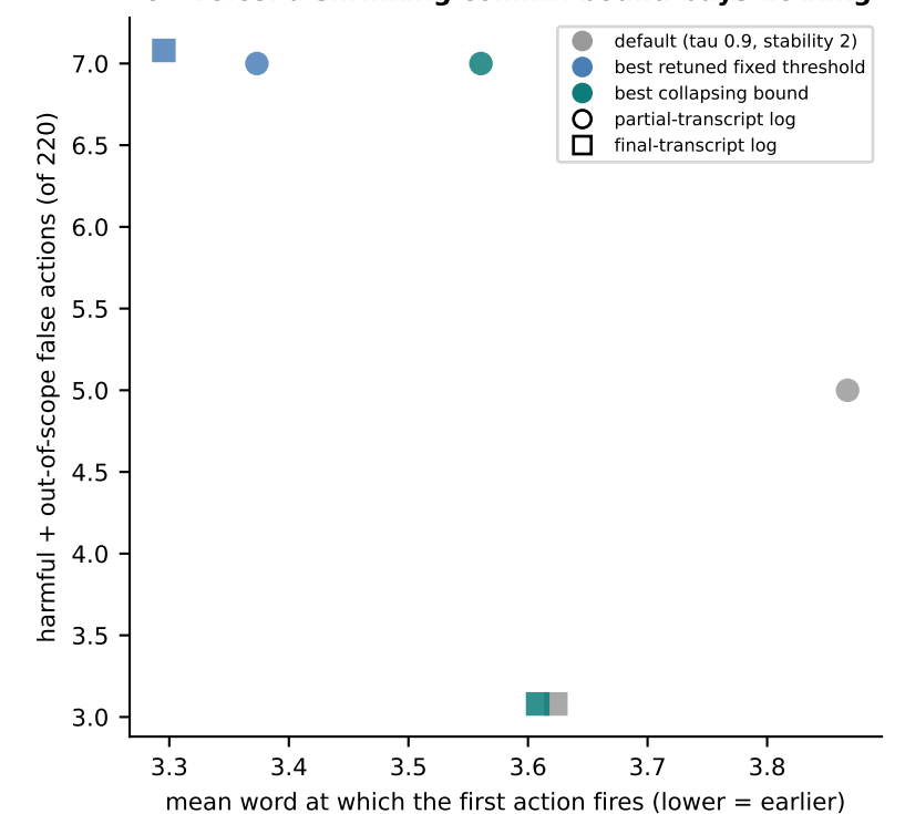
o • Voice: a shrinking commit bound buys nothing
