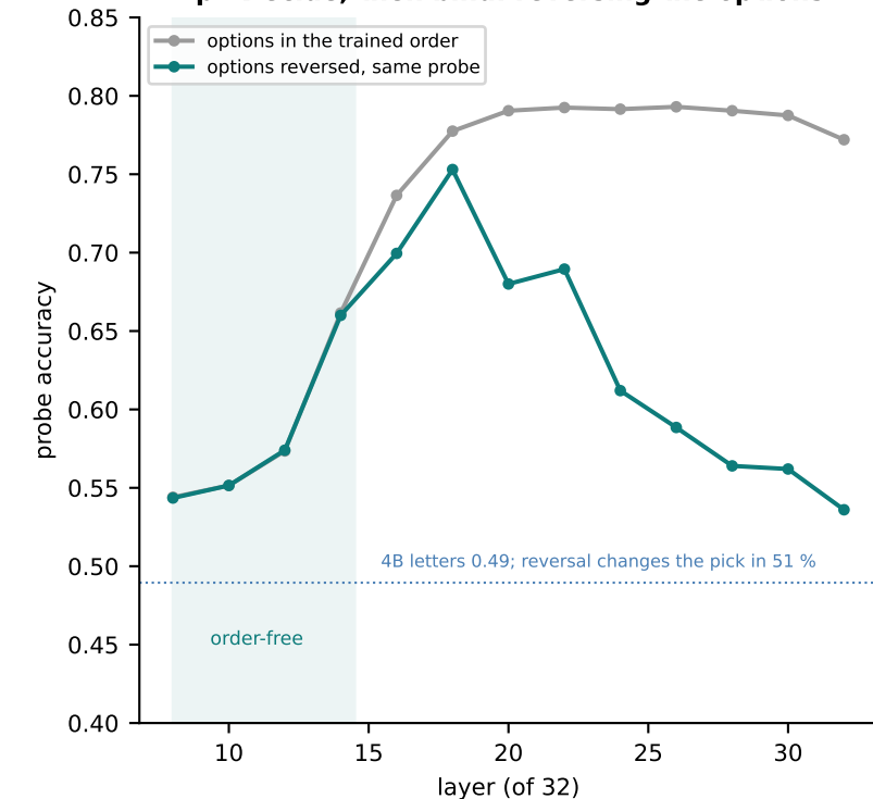
p • Decide, then bind: reversing the options
