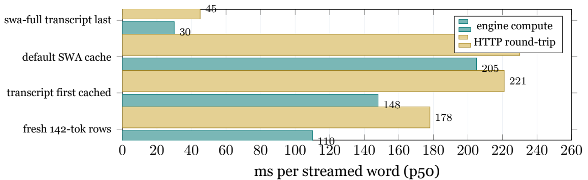
Figure 7: Same model, same readout: the 7× comes from layout and cache configuration, not from a smaller model.
