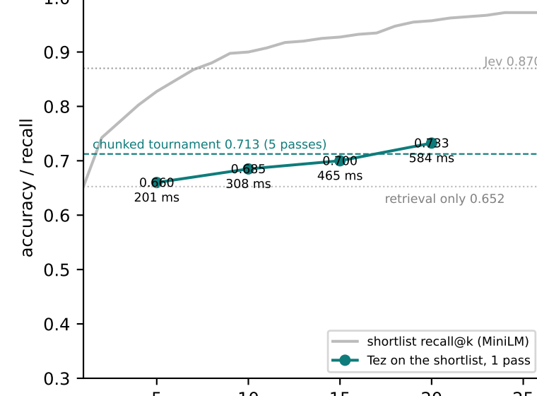
W · Banking77: shortlist, then decide
