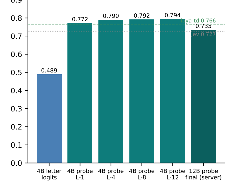
S · Probes on frozen hidden states (typed-decisions)
