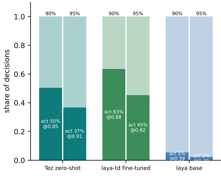
K · Conformal act / escalate (typed-decisions)
