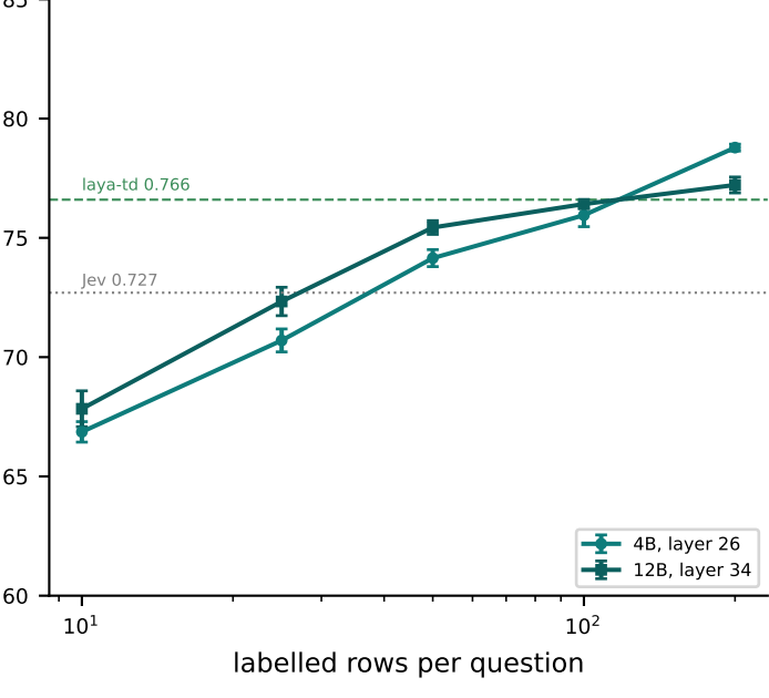
U · Probe data efficiency
