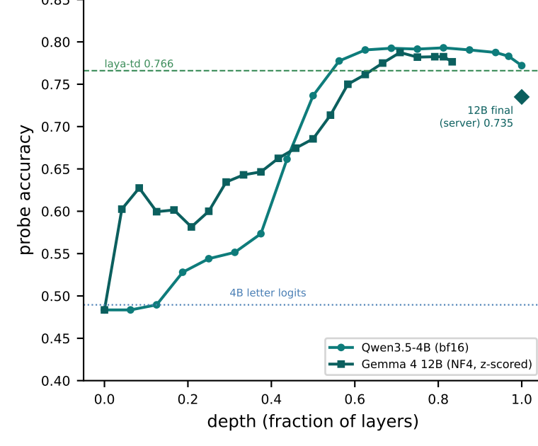
T · Probe accuracy by depth, 4B vs 12B
