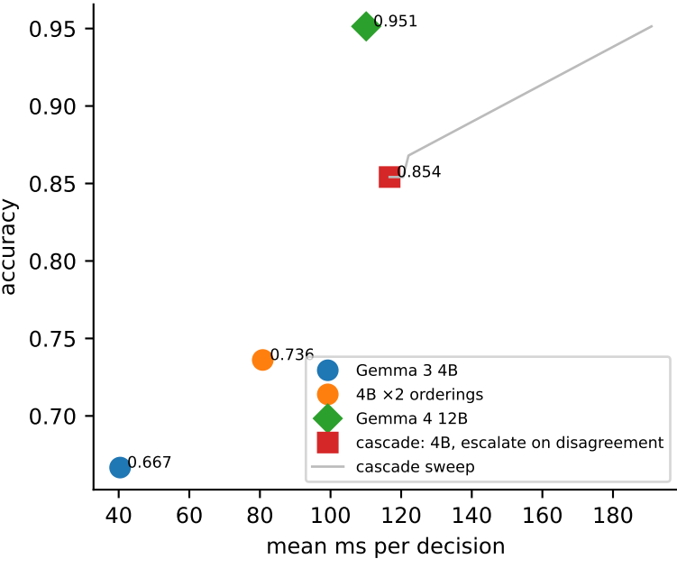
O · Small → large cascade: not worth it
