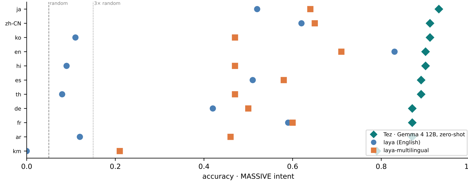
C · One frozen decoder vs two trained encoders, per language
