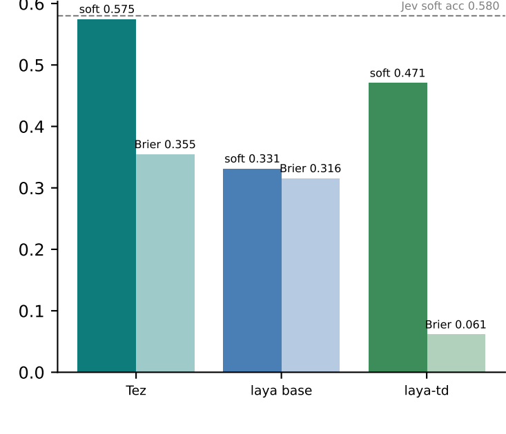
R · Teacher-distribution match (soft acc ↑, Brier ↓)
