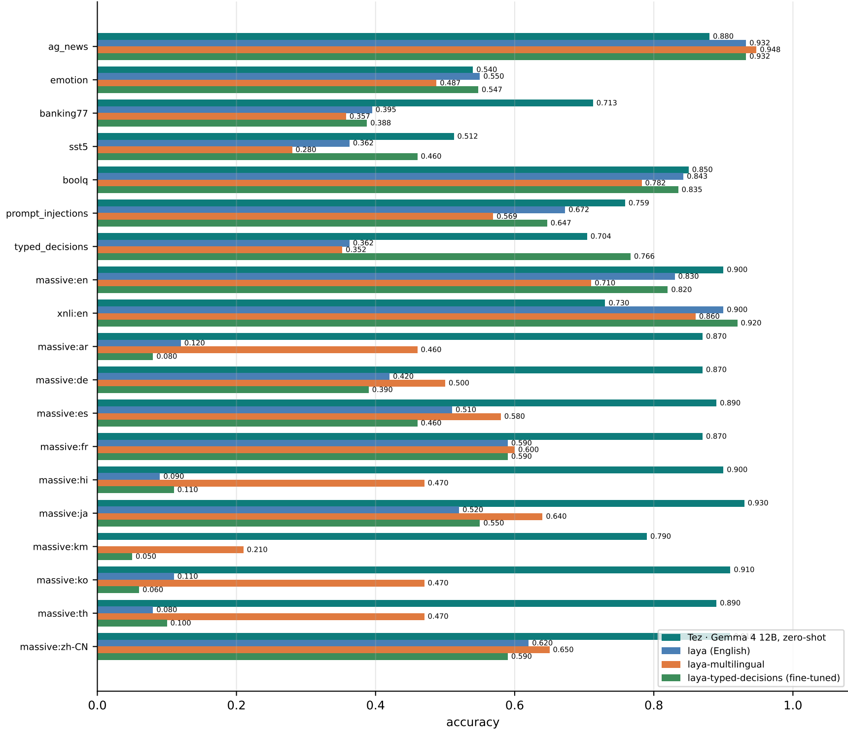
B · Every task, every checkpoint (MASSIVE: 20 options, 100/lang)
