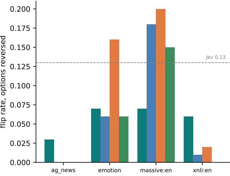
F · Option-order robustness (first 100 rows)
