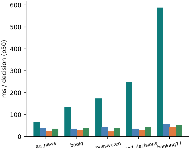
G · Latency, same GPU (Tez over HTTP, state uncached)
