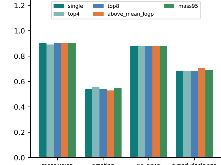
Y · Option elimination: no gain
