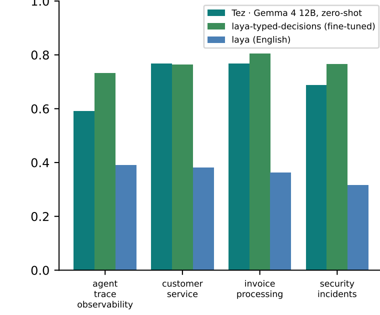
Q · typed-decisions by workflow
