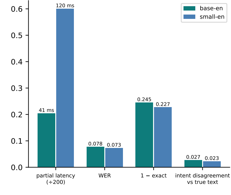
P · ASR stage (faster-whisper, synthetic speech)
