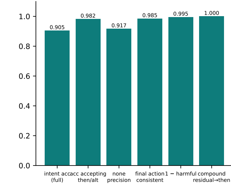
M · Voice → action outcomes (220 commands)
