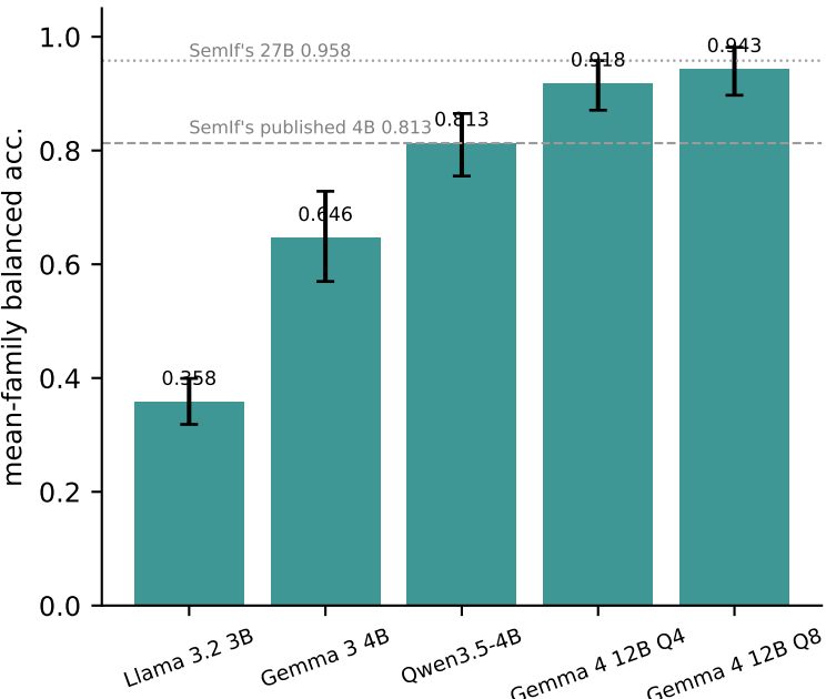
H · Scale-gated symbol binding (SemIf, 95% CI)
