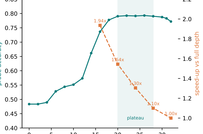
V · Early readout: probe accuracy vs prefill speed-up (4B)
