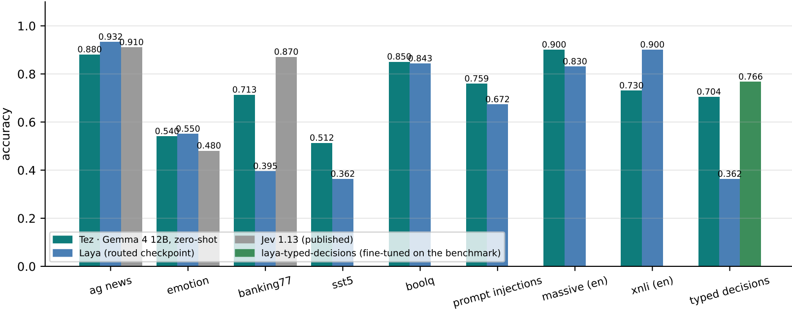
A · Accuracy on Laya's public datasets — same rows, same machine
