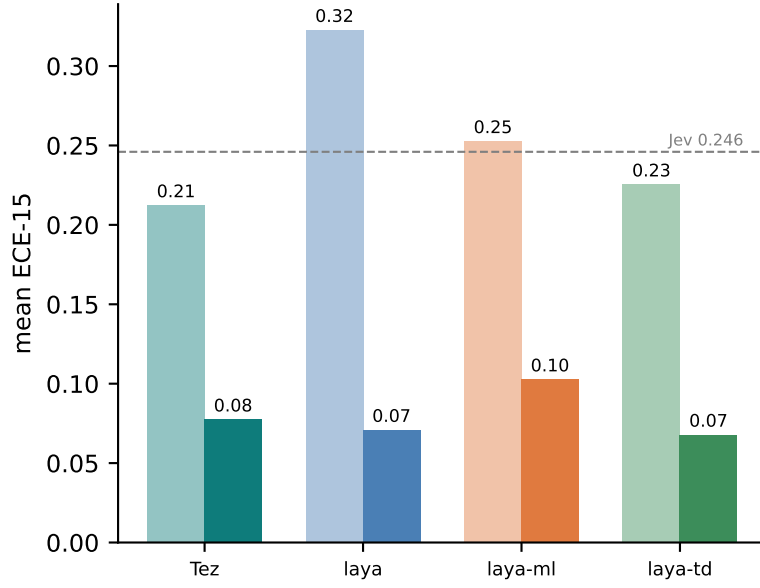
E · Calibration: shipped (light) → per-task refit (dark)
