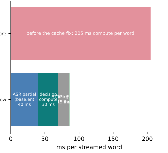
N · Per-word budget (~85 ms word → action)
