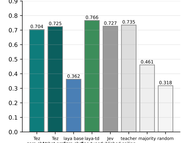
D · typed-decisions (2,000 decisions)
