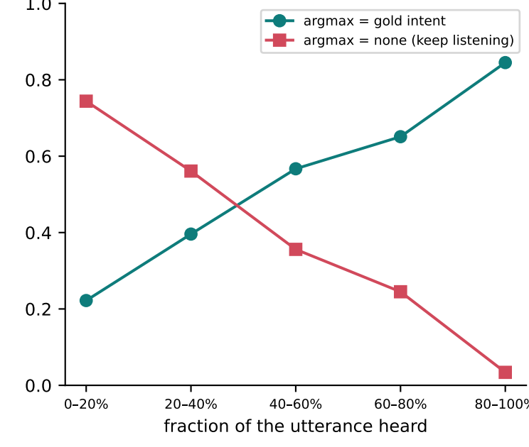
L · Voice: partial-transcript predictions
