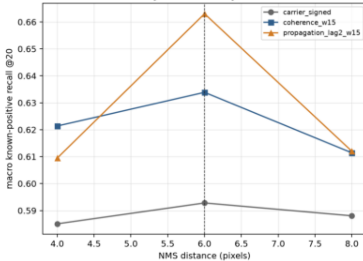
Primary and sensitivity NMS radii
