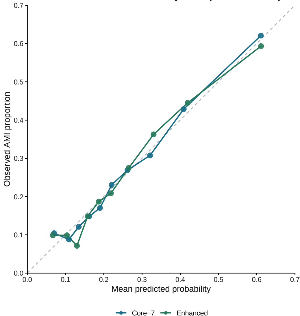
Calibration from mean 5-fold by 10-repeat held-out predictions
