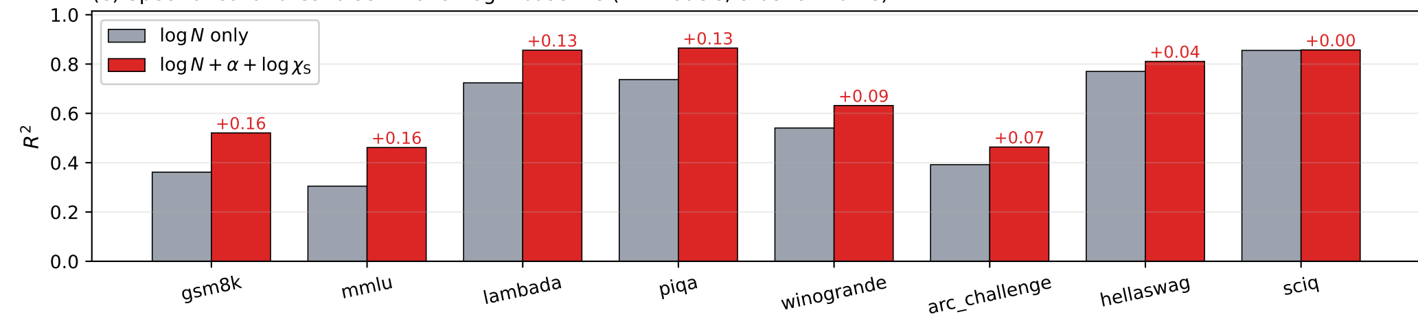
(e) Spectral covariates raise R^2 over \log N baseline (41 models, 8 benchmarks)
