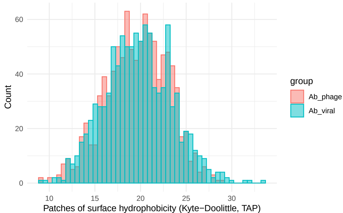
psh_15_kd: phage vs viral
