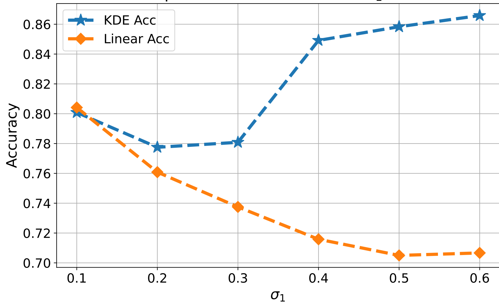
Comparison of Accuracies for \nu_1 = 0.3
