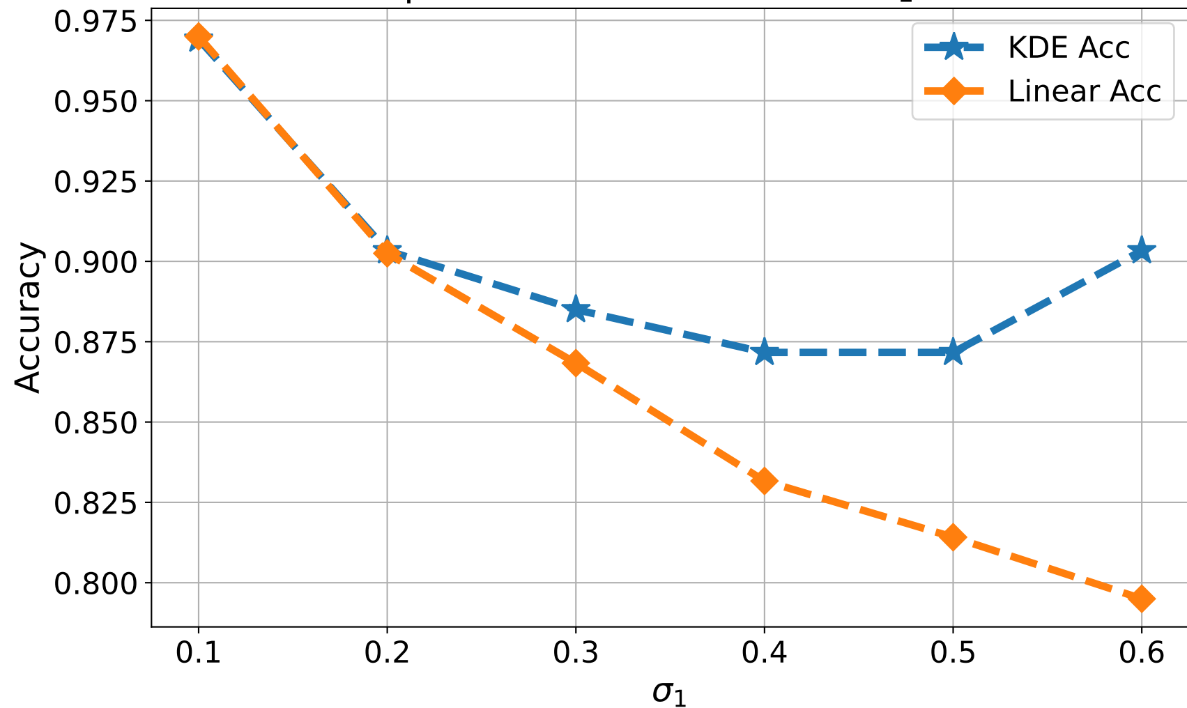
Comparison of Accuracies for \nu_1 = 0.5
