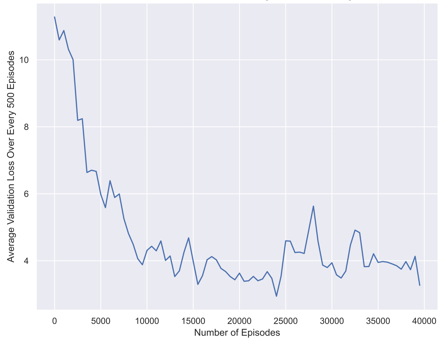
Decrease of Validation Loss During Double Q-Learning
