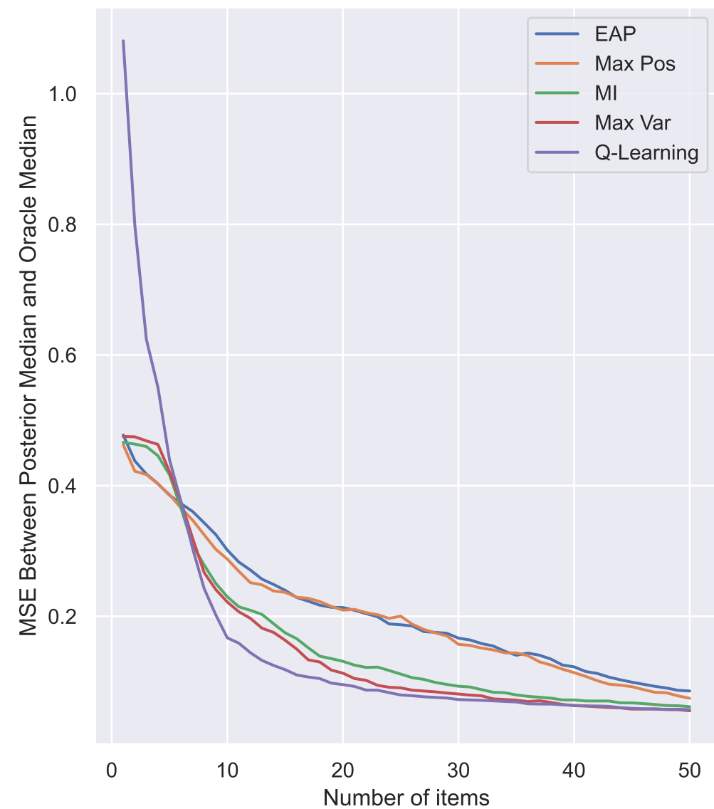
Dim 1: Number of Items v.s Estimation MSE
