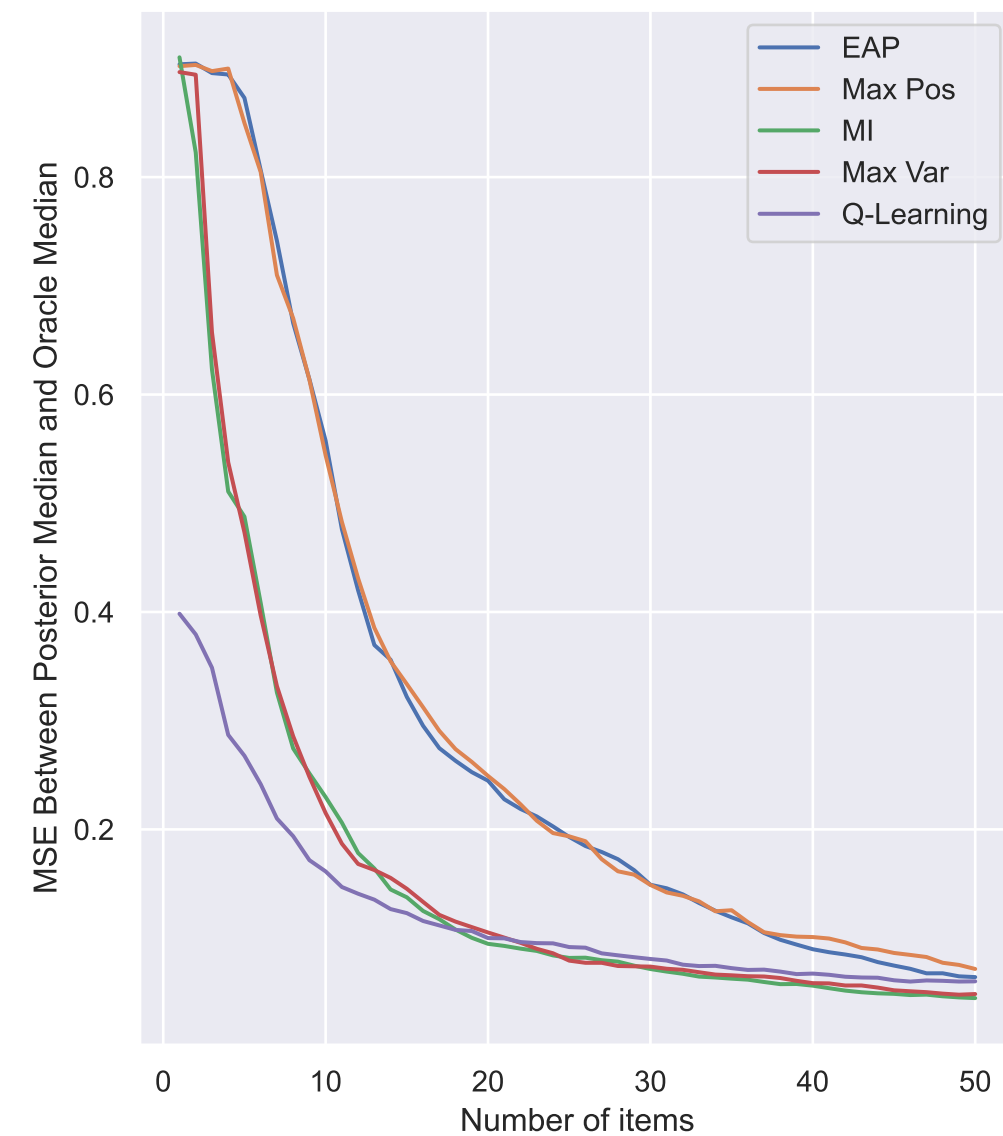
Dim 2: Number of Items v.s Estimation MSE
