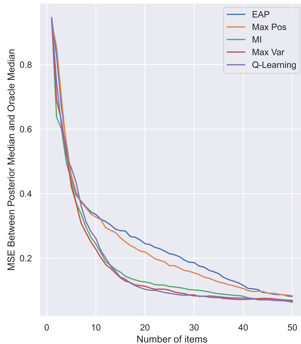
Dim 0: Number of Items v.s Estimation MSE
