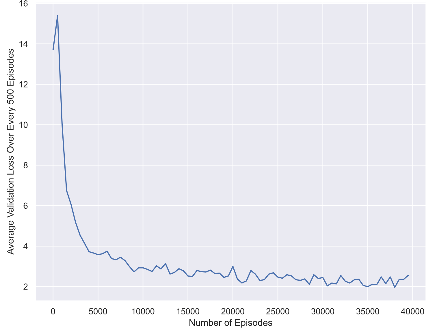
Decrease of Validation Loss During Double Q-Learning
