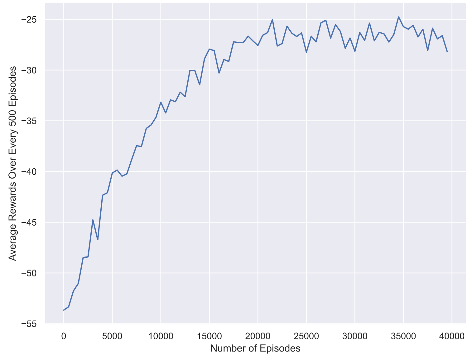
Increase of Rewards During Double Q-Learning
