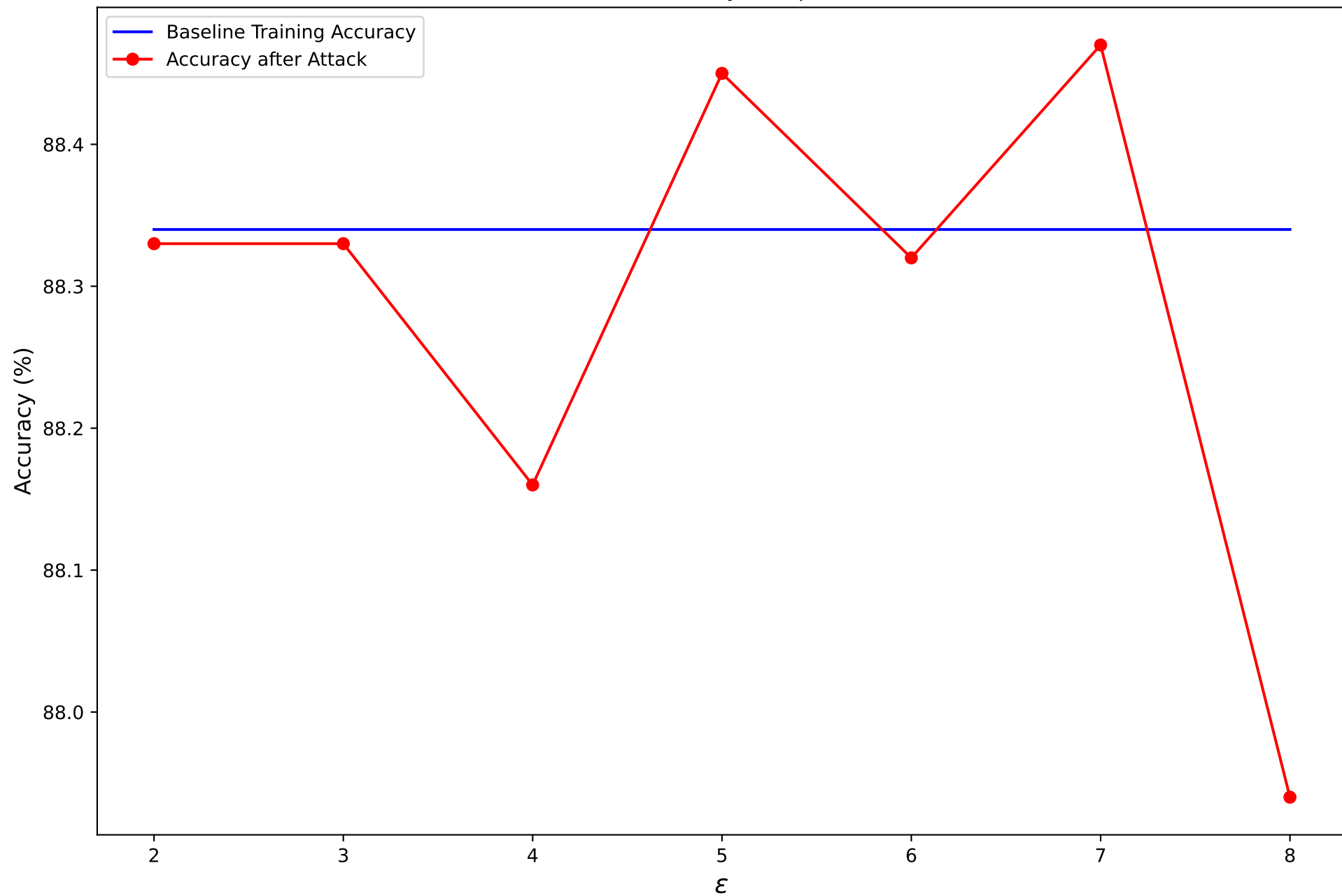
Model Accuracy Comparison
