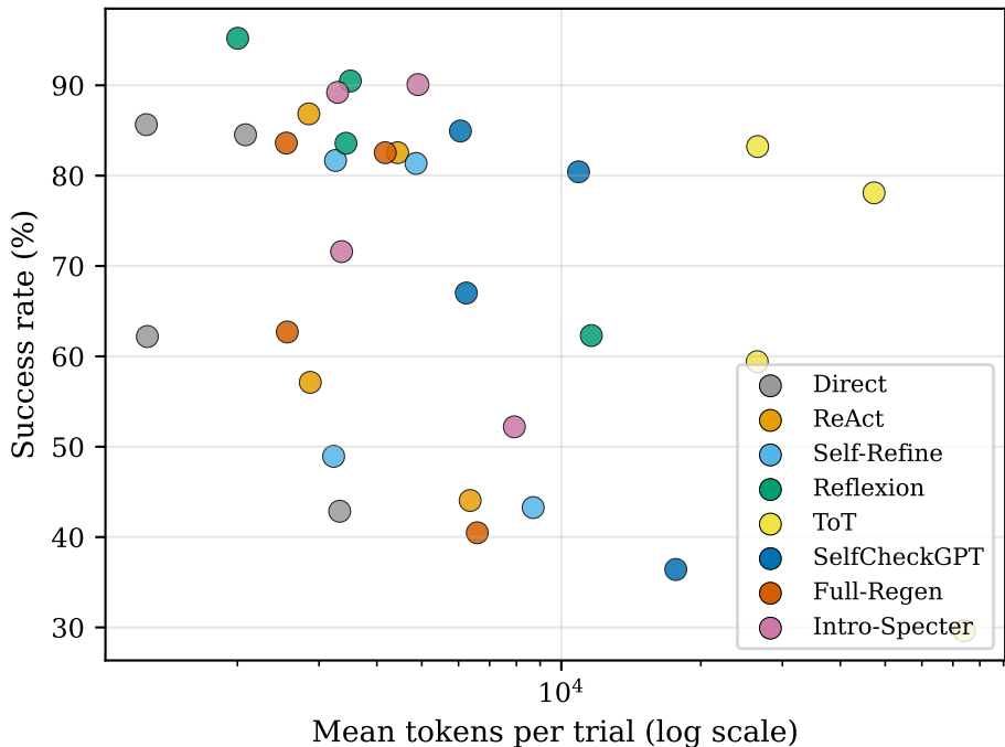
Token cost vs success — IS targets the upper-left quadrant
