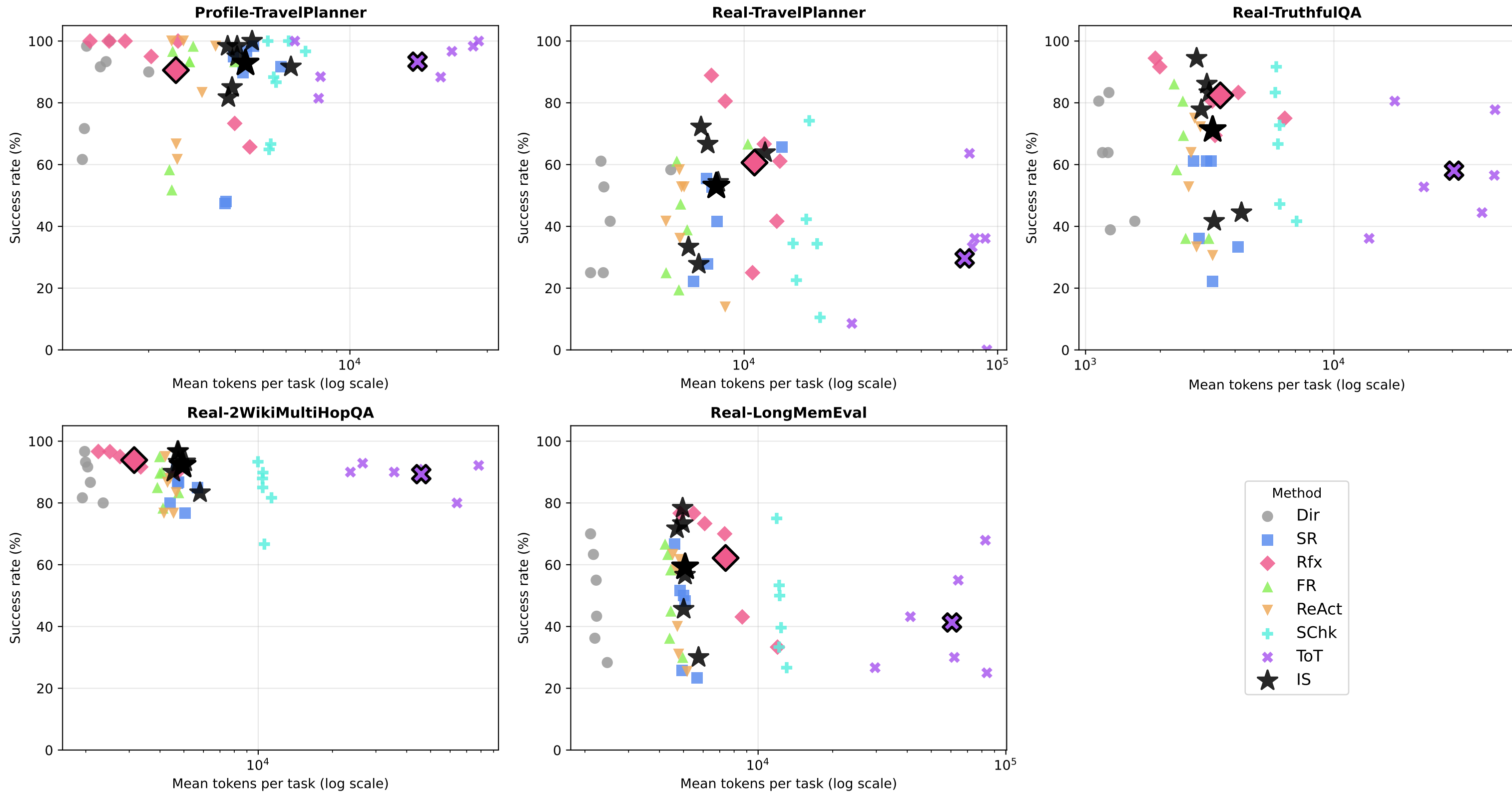
Cost-Accuracy Pareto across 5 Datasets × 6-7 LLMs × 8 Methods (IS = filled black star; large markers = method mean across LLMs)
