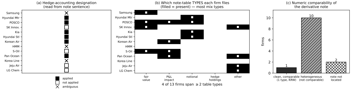
Figure 1: Live OpenDART extraction (FY2023 pilot), in black and white. (a) Hedge-accounting designation read from each firm’s note sentence: applied (filled), not applied (open), ambiguous ( \times ); the one robustly extractable outcome. (b) Which note-table types each firm files (filled cell = present); most firms span two or more, so a single parser cannot align them. (c) Numeric comparability of the derivative note: only one of thirteen located notes is a clean single-type table.
