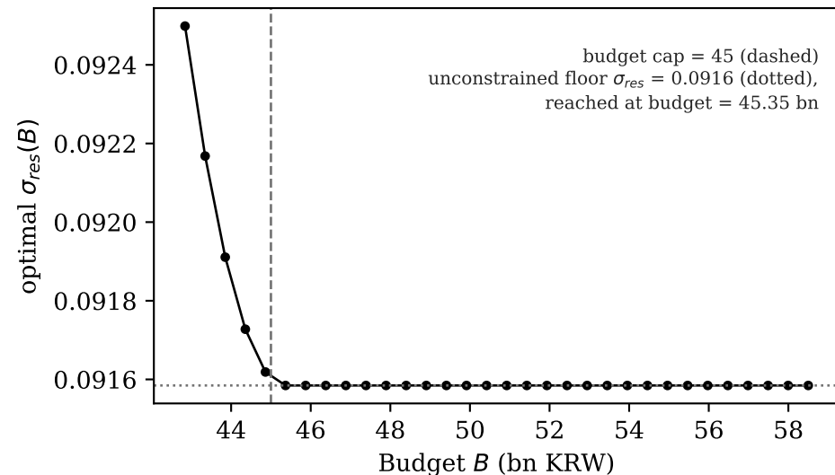
European (Black-76 / GK premiums)
