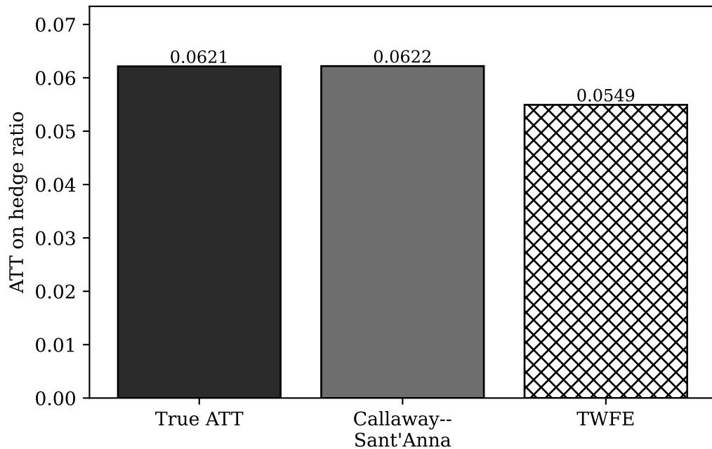
(b) CS recovers the truth; TWFE biased under dynamic, staggered timing
