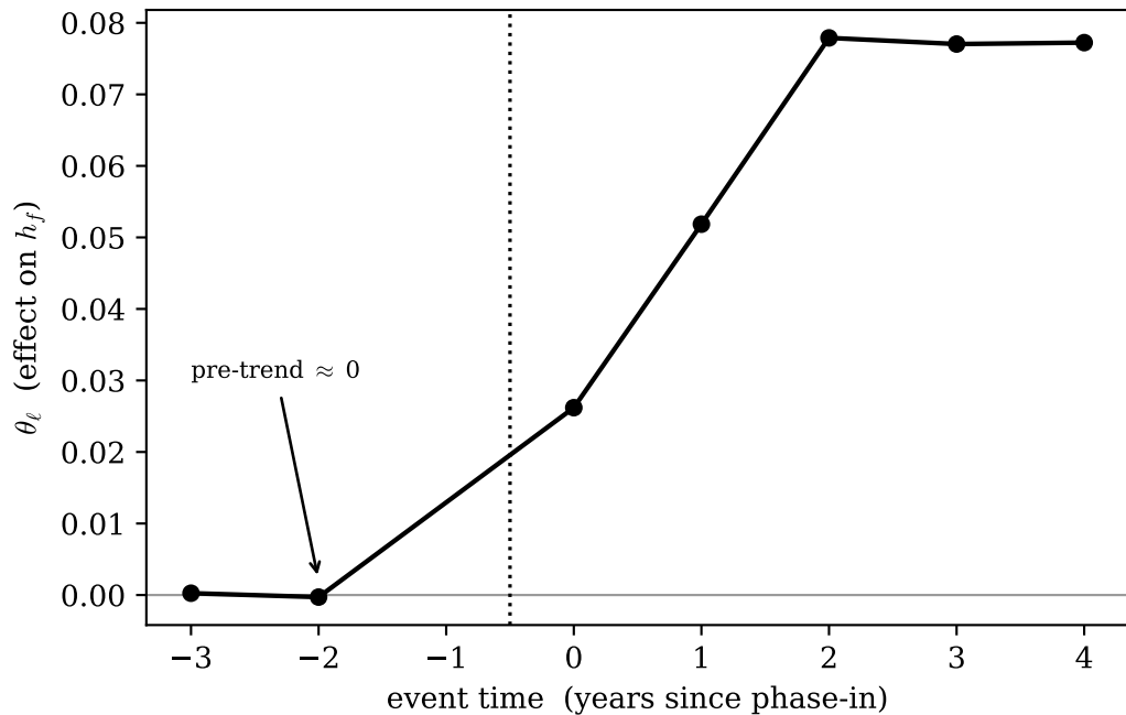
(a) Event study: flat pre-trend, effect ramps in
