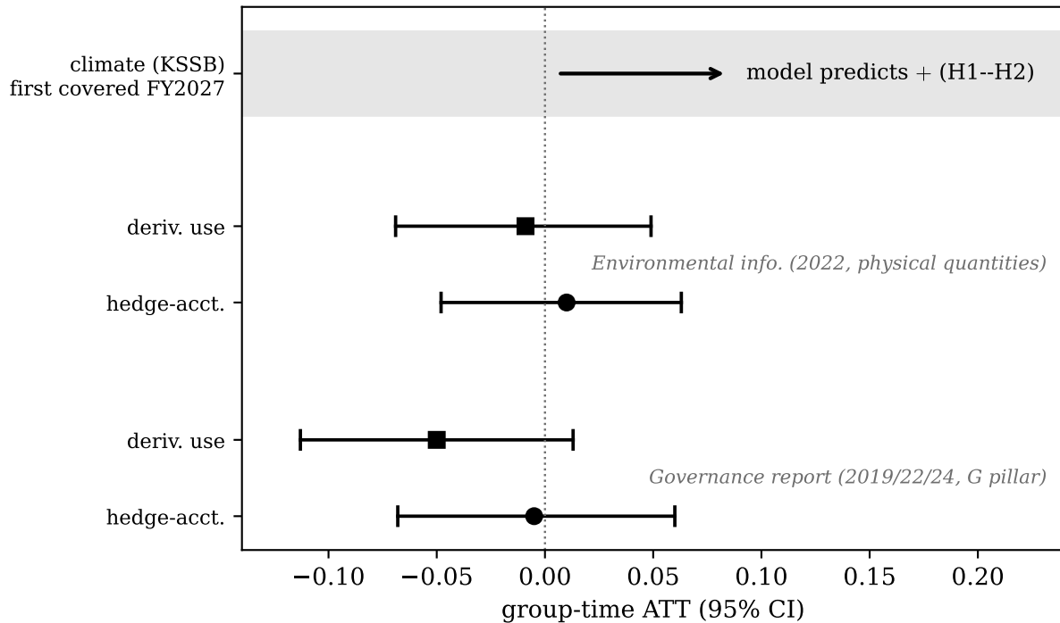
(a) the exposure ladder: nulls below, prediction on top
