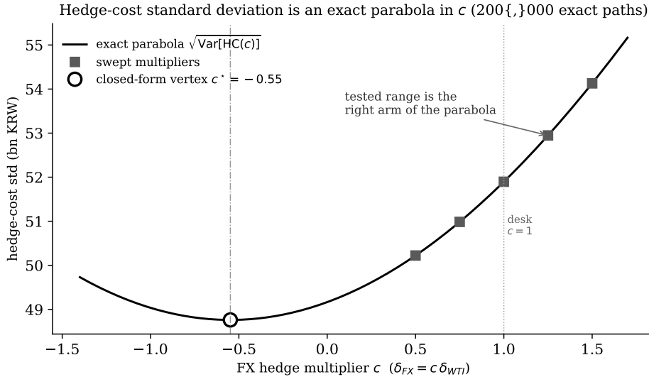
Figure 8: Hedge-cost standard deviation as the rigorous parabola \sqrt{\text{Var}[\text{HC}(c)]} implied by the affine decomposition (25), computed at 200,000 jump-adapted rigorous paths (Section 8.3). The five swept multipliers (Table 6) lie on the parabola’s right arm; the natural reference point c = 1 sits well up that arm, and the closed-form vertex c^* = -0.55 (27), the variance minimizer, lies to the left of the entire tested range.
