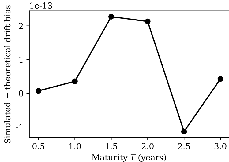
Closed-form P/Q drift-bias check (agreement to numerical tolerance)
