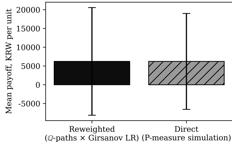
Girsanov reweighting vs. direct P-sim (residual = 0.11% of direct mean)
