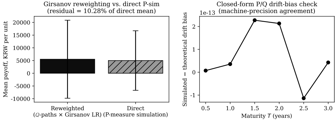
Figure 11: Left: Girsanov-reweighted vs. direct-simulation mean payoff on the actual KO structure. Right: exact machine-precision agreement of the corresponding closed-form drift-bias test (Table 9).
