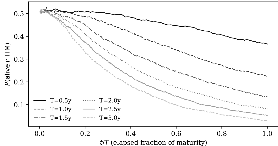
Alive-and-ITM path probability decay, by maturity
