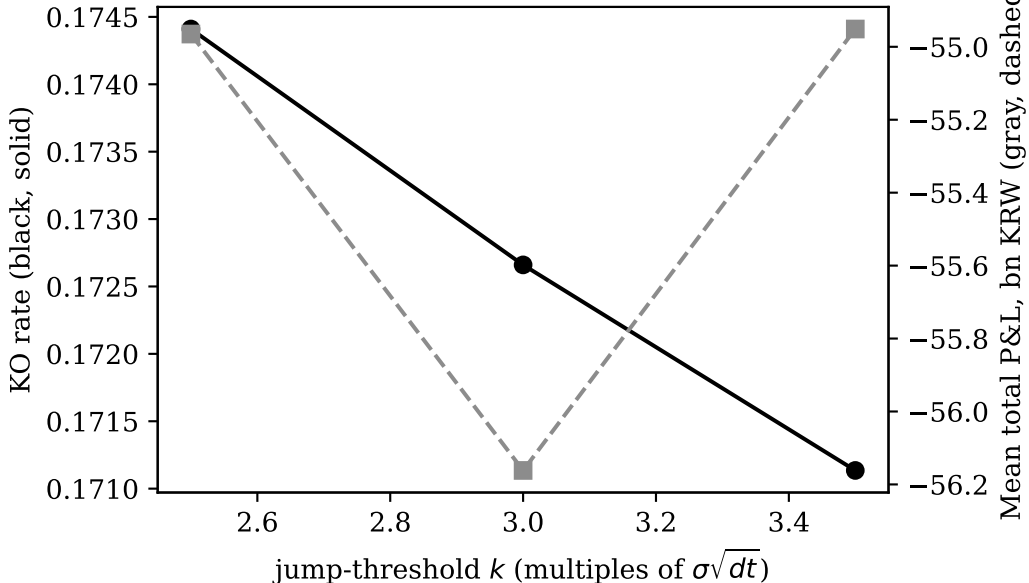
k -sigma threshold robustness ( n = 200,000 exact paths)
