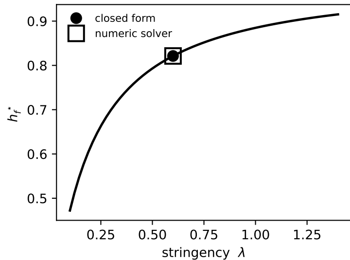
(a) \partial h_f^* / \partial \lambda > 0 (H1)
