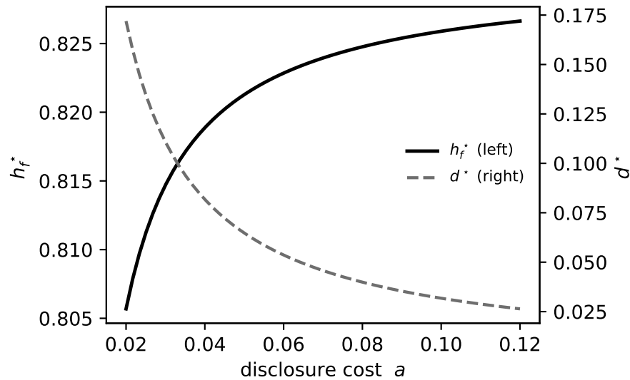
(b) \partial h_f^* / \partial a > 0, \partial d^* / \partial a < 0 ( H_{\text{sub}} )
