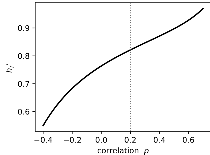
(c) sign of \partial h_f^* / \partial \rho per Eq.(20)
