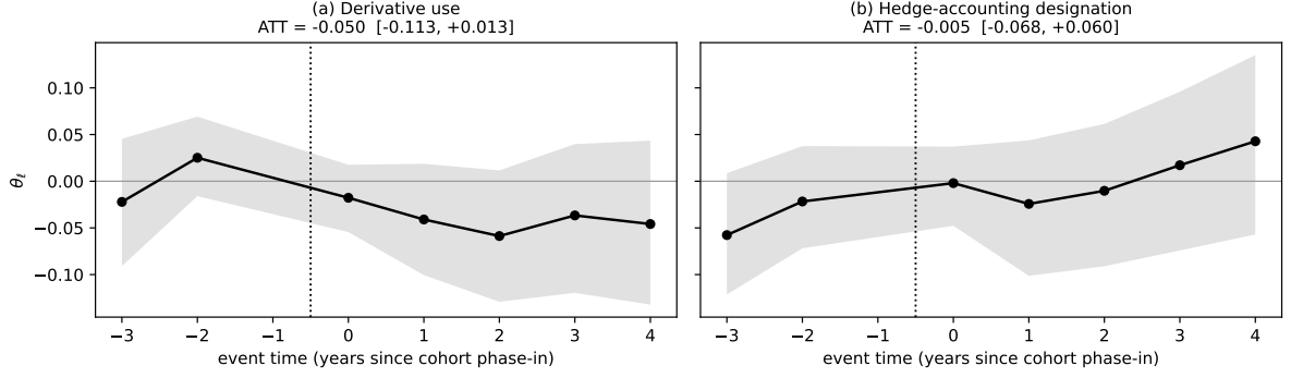
Figure 2: Event studies (380-firm panel; shaded areas are 95% bootstrap bands): (a) derivative use, (b) hedge-accounting designation. Both paths are flat through the phase-in.
