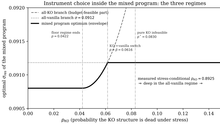
Figure 5: The mixed program's optimal residual volatility as a function of p_{KO} , with its two branches, using the independently-priced standalone KO premium. Floor regime ( p_{KO} \leq 0.0422 ): the all-KO ledger leaves the budget slack and the unconstrained variance floor 0.0908 is attained. Budget-pinned KO regime (0.0422–0.0616): achieved risk deteriorates as mortality consumes the ledger. All-vanilla regime ( p_{KO} \geq \bar{p} = 0.0616 ): the book switches instruments and the optimum is invariant at 0.0912. The measured stress-conditional p_{KO} = 0.8925 lies far inside the vanilla regime.
