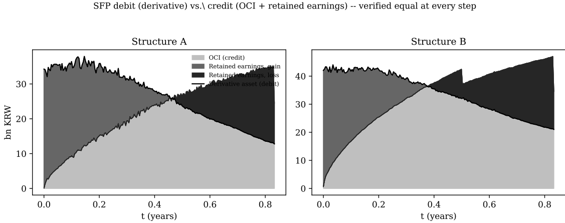
Figure 8: SFP debit (derivative asset, black outline) vs. credit (OCI reserve plus retained earnings, stacked area) over time, Structure A and Structure B. The outline traces the top of the stacked area at every step by construction (Eq. 34). Structure B’s visible kink near t \approx 0.5 is the maturity-freeze plateau of Section 8.6.
