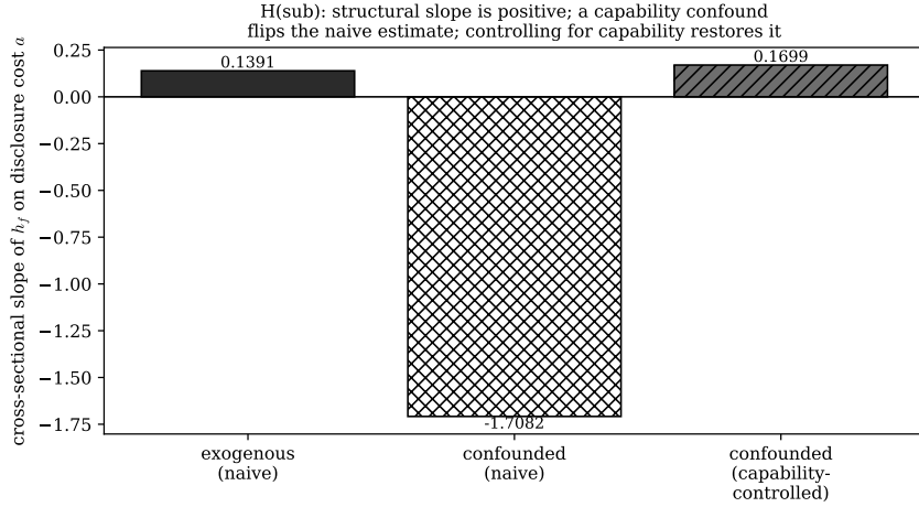
Figure 8: H(\text{sub}) fragility. Cross-sectional slope of treated-firm hedging on disclosure cost a : positive when a is exogenous (structural \partial h_f^*/\partial a > 0 ), flipped negative by a capability confound, restored positive by controlling for capability. The substitution channel is real but second-order, hence identifiable only with the safeguards of Section 4.
