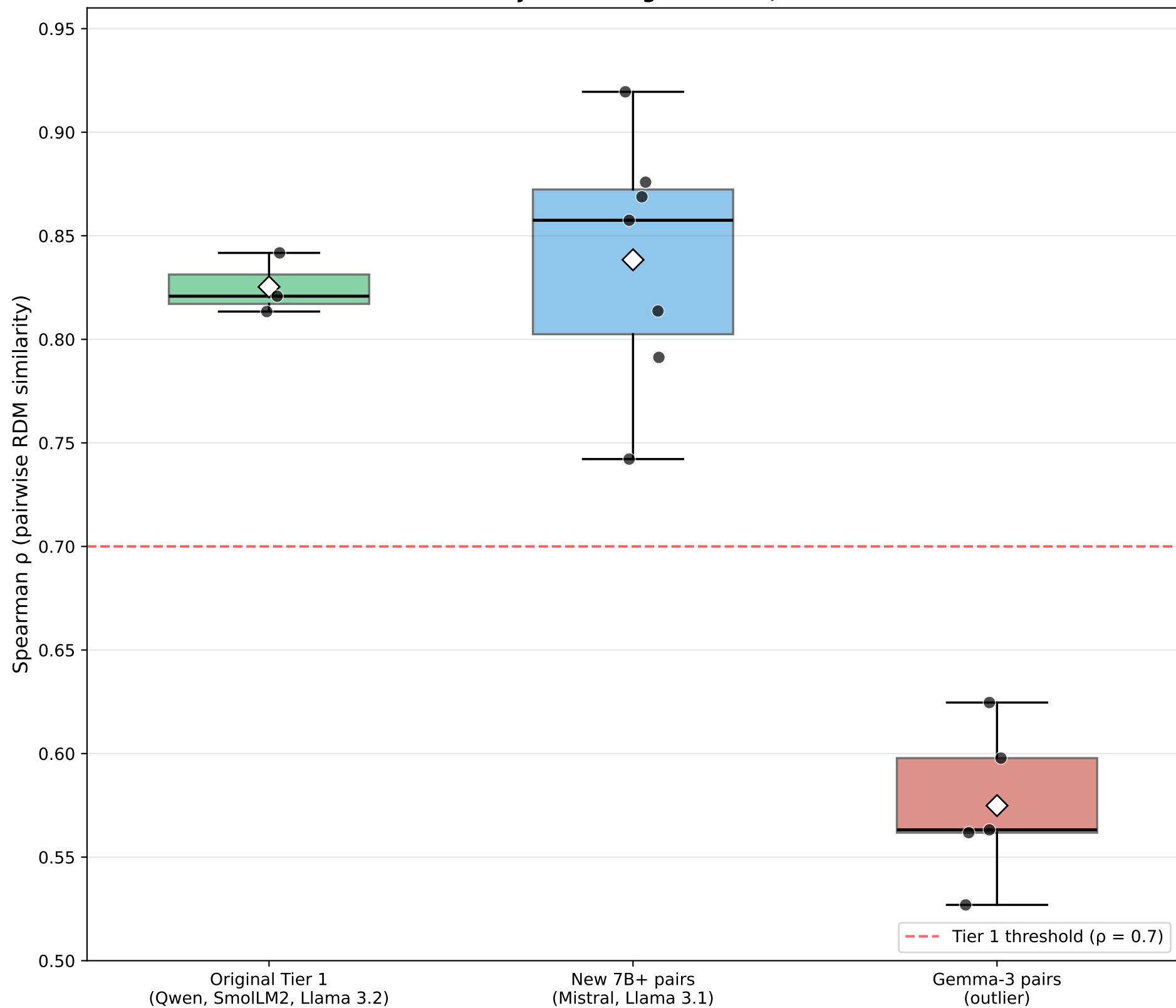
Tier 1 Cluster Re-Verification (n = 12, instruct only) Mistral 7B and Llama 3.1 8B join the original Tier 1; Gemma-3 remains outlier
