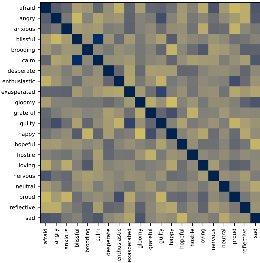
Qwen 2.5 1.5B Instruct (Compliance-yielding: B=0.80, D=0.61)
