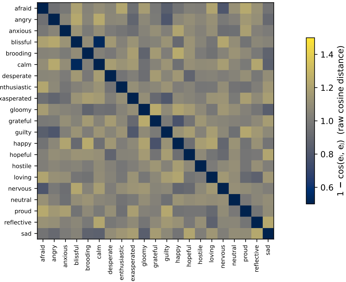
Llama 3.2 3B Instruct (Compliance-refusing: B=0.20, D=0.85)
