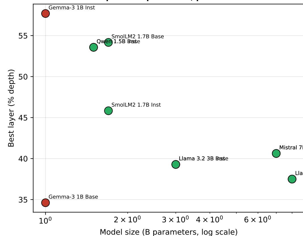
(C) Best Layer Depth vs Size Spearman \rho = -0.484 , p = 0.111
