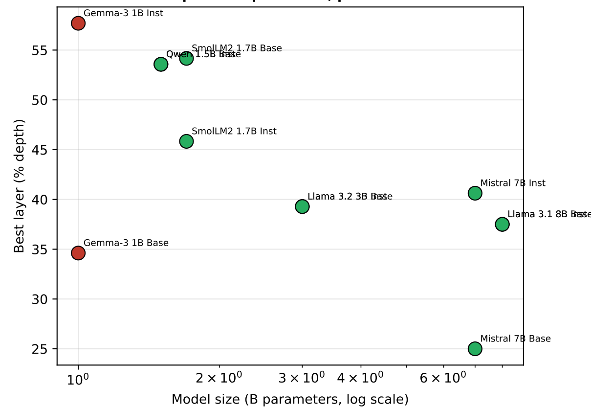
(C) Best Layer Depth vs Size Spearman \rho = -0.540 , p = 0.070
