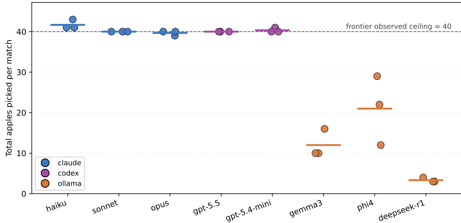
Commons-harvest yield gap (all matches sustainable, no tree death) frontier ~40 vs ollama 3-29 — a yield gap at the same sustainability
