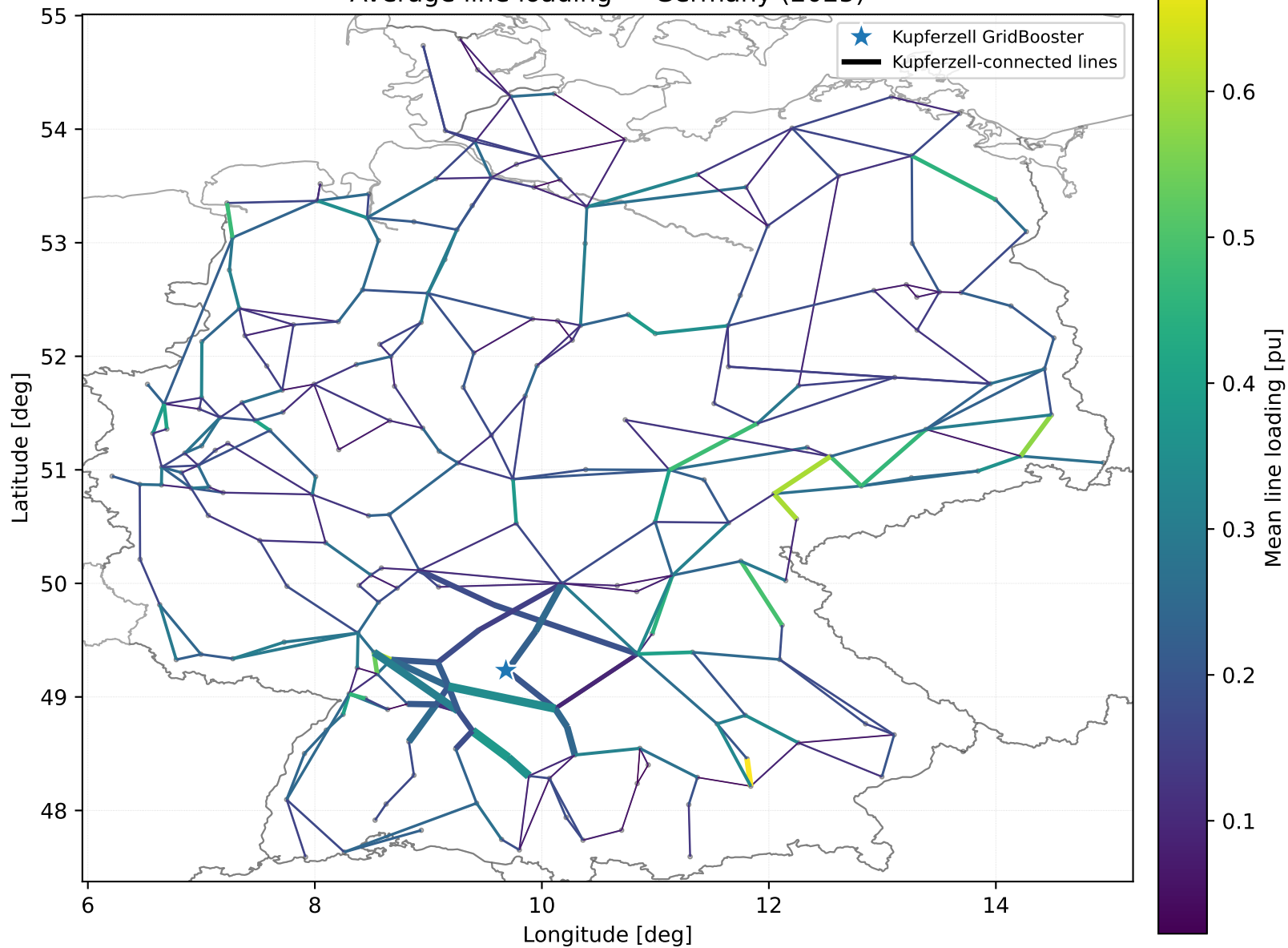
Average line loading — Germany (2025)
